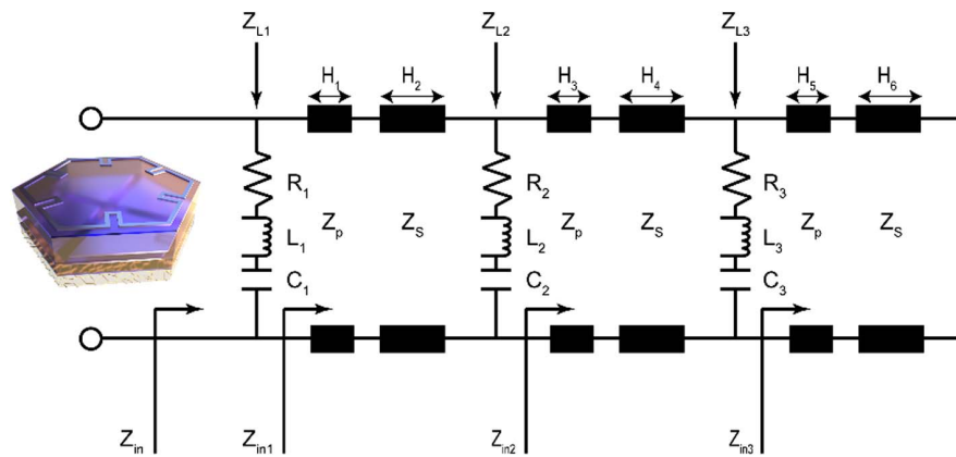
Fig. 13. Equivalent circuit model of the OTMMA.
