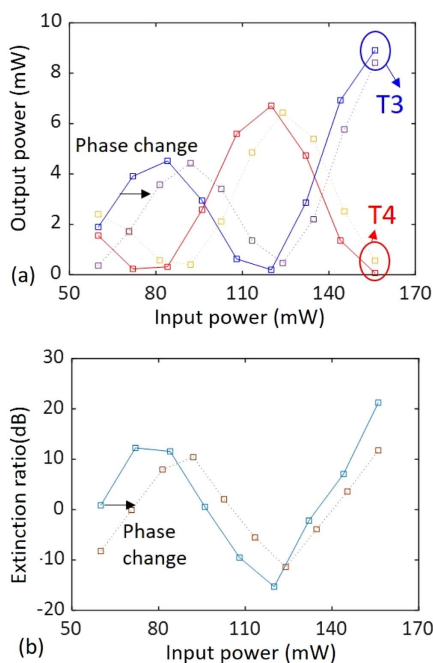
Fig. 6. Experimental results of the NMZI switch with the input of a pulsed light source: (a) output powers versus input powers at T3 and T4; (b) T3-to-T4 extinction ratio in dB.
