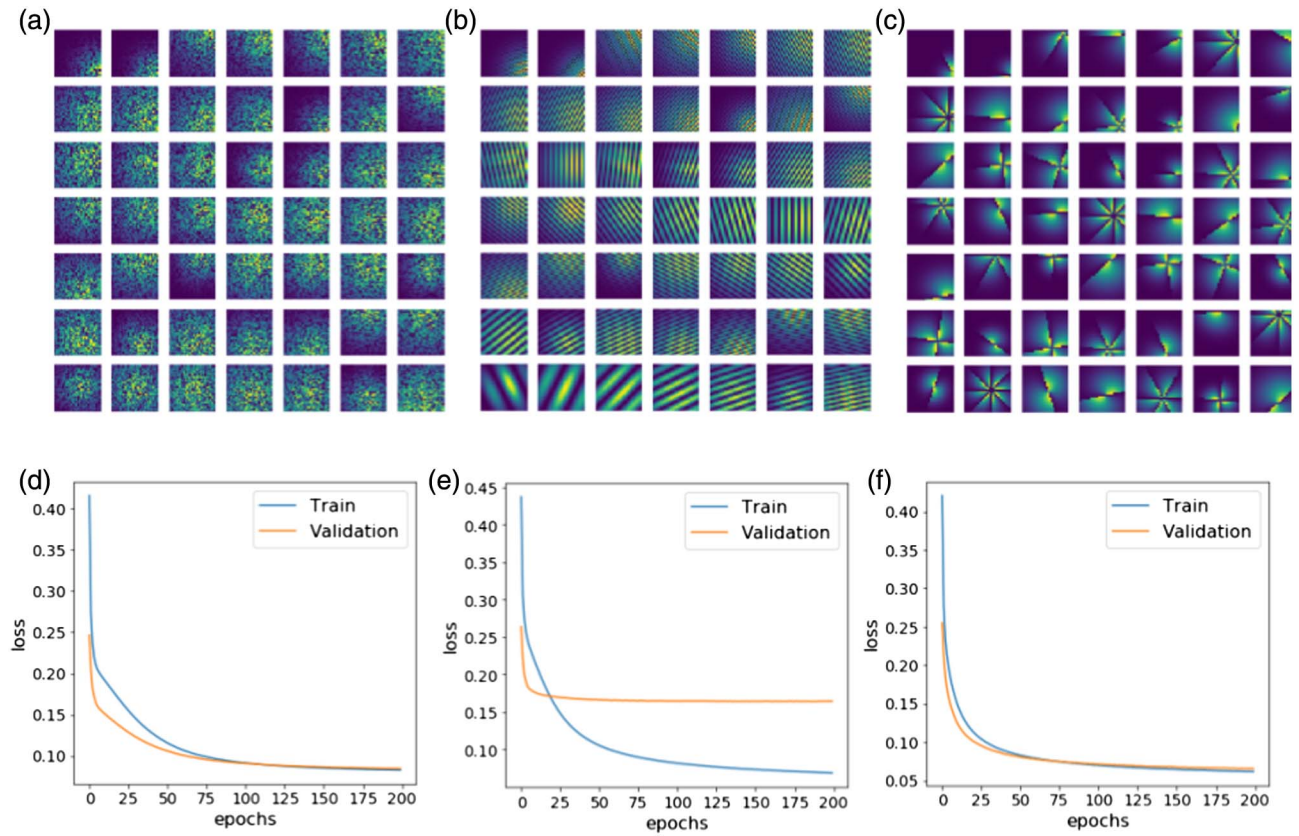
Fig. 3. (a)–(c) Sample training images X_R , X_F , and X_V or random, Fourier, and vortex training sets. (d)–(f) Corresponding training and validation curves.
