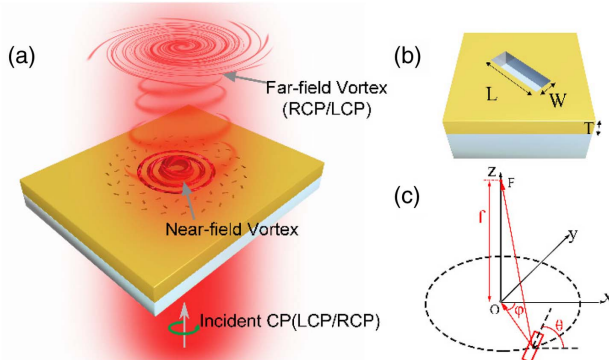
Fig. 1. Bi-channel optical vortex generated in both the near and far fields. (a) Schematic of NFVG that is based on a plasmonic metasurface which consists of a nanoslit array. (b) The nanoslit on an Au film works as the building block of NFVG with width W = 80 nm, length L = 250 nm, and depth T = 120 nm. The depth T is also the thickness of the Au film. (c) Schematic diagram that illustrates the design principle of the bi-channel metasurface using geometric phase of the nanoslit in both the near and far fields. Under illumination of CP light with a specific spin state (LCP/RCP), the proposed metasurface can simultaneously generate focused SP vortex at the center (point O ) of the metasurface and focused far-field vortex (cross-polarization, RCP/LCP) of scattered light at point F with a designed focal length f .
