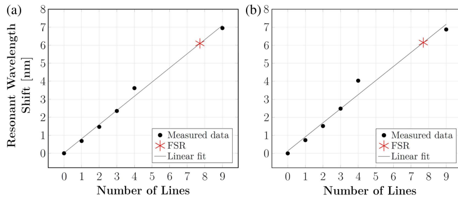
Fig. 5. Dependence of the resonant wavelength shift on the number of lines written across the racetrack. For each line, an arc length of approximately 14 \mu\text{m} has been exposed. (a) Device without oxide cladding and (b) device with oxide cladding.
