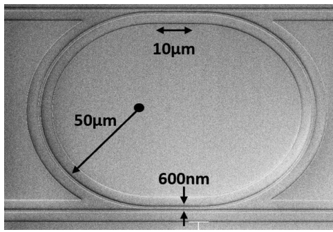
Fig. 1. SEM image of one of the resonators.
