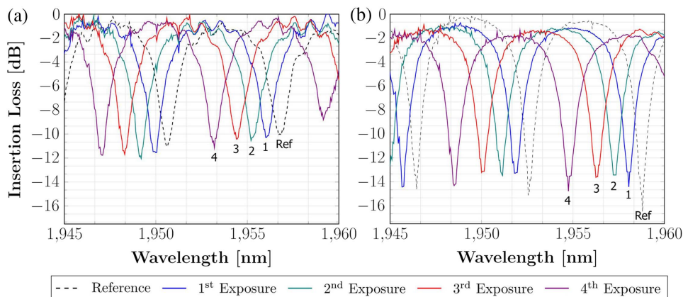
Fig. 4. Transmission spectra of fabricated racetrack resonators for different lengths of the exposed section of the resonator. (a) Device without oxide cladding and (b) device with oxide cladding.
