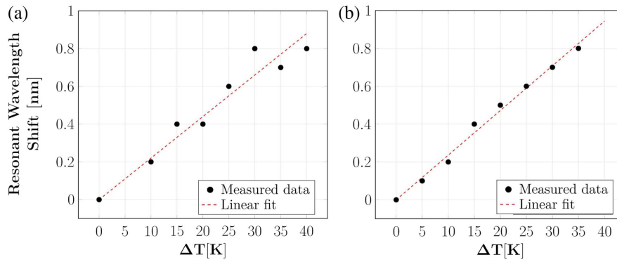
Fig. 7. Measured resonant wavelength shift as a function of change in the ambient temperature. (a) Device without oxide cladding and (b) device with top oxide cladding.
