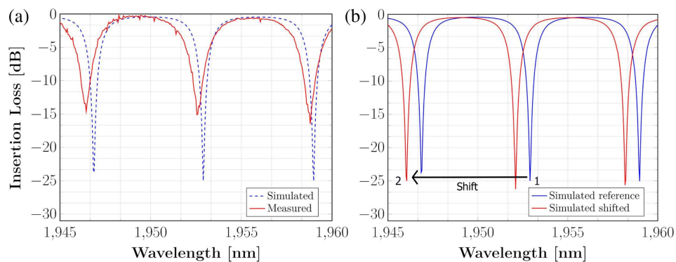
Fig. 6. (a) Transmission spectra of the simulated device, compared to the measured spectrum. (b) Transmission spectra obtained by simulation, before and after changing the refractive index of silicon nitride.
