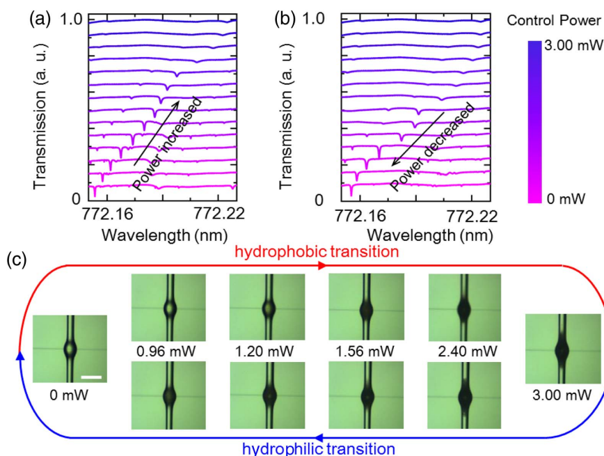
Fig. 2. Transmission evolution of the microbubble with the PNIPA hydrogel when the control power of the irradiation light first (a) increases from 0 to 3.00 mW, and then (b) decreases from 3.00 to 0 mW; (c) CCD images of a cycle of phase-transition process of the PNIPA hydrogel. The microbubble changes from transparent hydrophilic state to opaque hydrophobic state due to the increased scattering. Inset, the scale bar is 125 μm.
