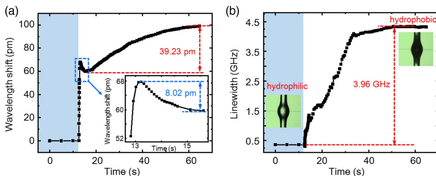
Fig. 4. (a) Real-time WGM resonance wavelength shift and (b) linewidth broadening during the PNIPA hydrogel phase transition (a hydrophilic to hydrophobic transition) monitored by an MBR. The control power of the irradiation light is switched on at ~12.5 s. During the whole phase-transition process, a small blueshift of 8.02 pm in wavelength is first observed within 13.22–15.62 s; then the overall redshift of the resonance wavelength is 39.23 pm, and the maximized linewidth broadening is 3.96 GHz.
