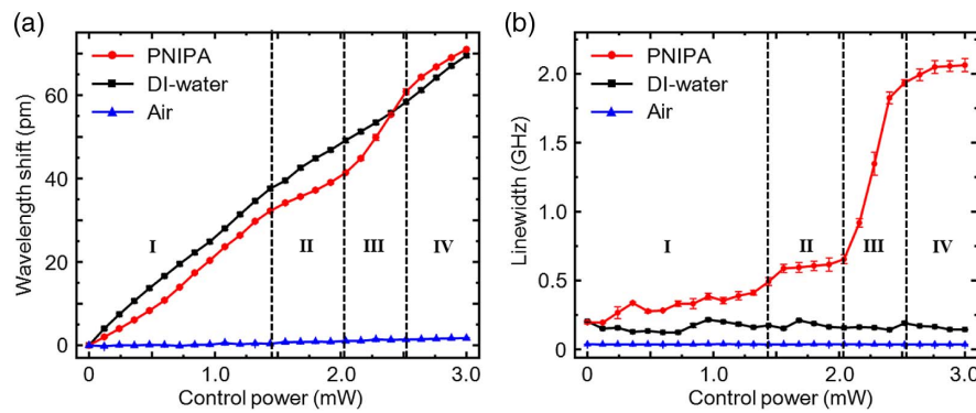
Fig. 3. (a) WGM wavelength shifts and (b) linewidth broadenings as a function of control power of the irradiation light from 0 to 3.00 mW, when the MBRs are filled with air (blue line with triangular marker), DI water (black line with square marker), and PNIPA hydrogel (red line with circular marker). Compared with the result of microbubble cavities filled with air and DI water, note that a hydrophilic to hydrophobic transition process of PNIPA can be clarified as four stages: (i) pure hydrophilic state (0–1.44 mW); (ii) subtransition state (1.44–2.04 mW); (iii) transition state (2.04–2.52 mW); (iv) pure hydrophobic state (>2.52 mW).
