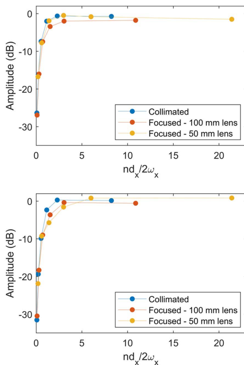
Fig. 3. Transmission amplitude as a function of the number of slits normalized by the beam diameter for the three different setup configurations, for sample thicknesses of (top) 102 \pm 1\text{ }\mu\text{m} and (bottom) 188 \pm 1\text{ }\mu\text{m} , at frequencies 0.48 THz and 0.44 THz, respectively.
