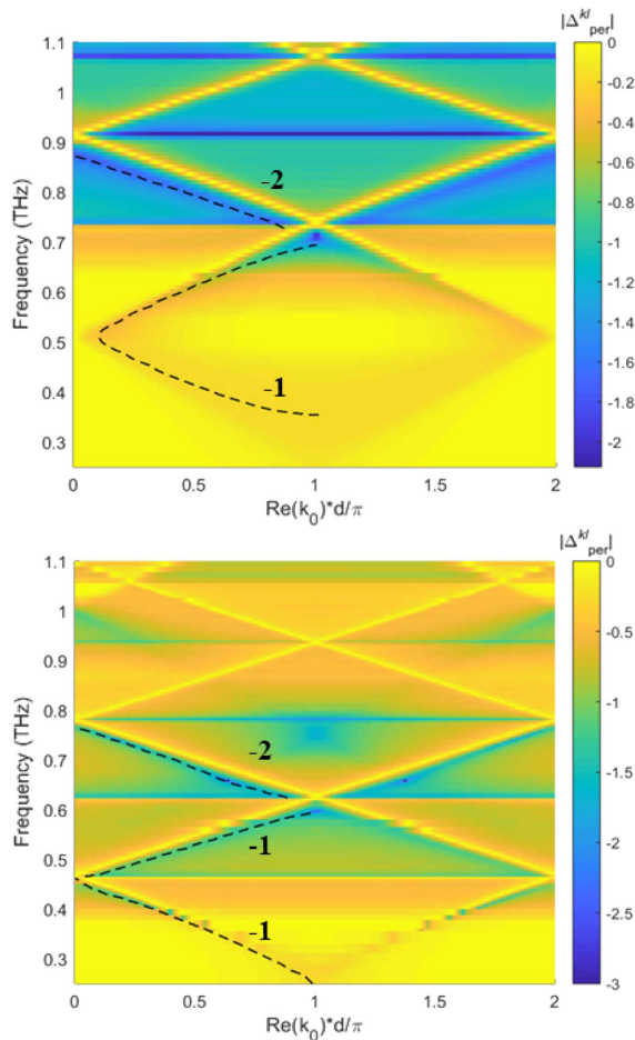
Fig. 13. Dispersion diagrams calculated from the method of moments for h = 102 \mu\text{m} (top) and h = 188 \mu\text{m} (bottom). The color represents the value of the determinant of the method of moments system in logarithm scale and the dashed lines indicate the modes, which are labeled according to their respective orders.
