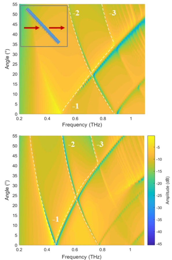
Fig. 14. Simulation of transmission through infinite periodic arrays with h = 102 \mu\text{m} (top) and h = 188 \mu\text{m} (bottom) using CST Microwave Studio unit cell boundary conditions and Floquet ports. The space harmonics calculated using method of moments are indicated by the white dashed lines. The inset presents a sketch of the simulation demonstrating the off-axis illumination and detection scheme. The blue and grey regions indicate the dielectric material and metal, respectively, while the red arrows indicate the direction of incident and transmitted radiation.
