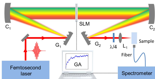
Fig. 1. Schematic of the experimental setup. G_1 and G_2 are two diffraction gratings of 1200 lines/mm each. C_1 and C_2 are two cylindrical concave mirrors each of focal length 200 mm. SLM, spatial light modulator; \lambda/4 , quarter-wave plate; L_1 , focusing lens; GA, genetic algorithm.
