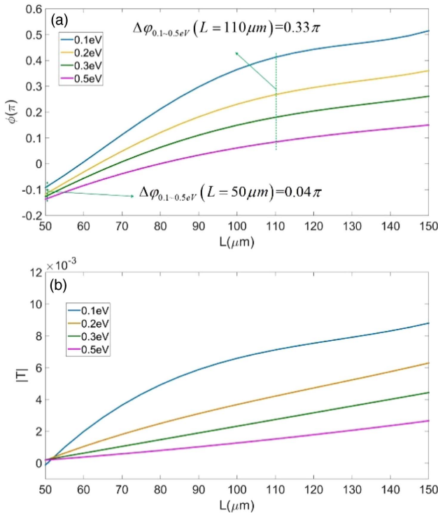
Fig. 2. Dependence of transmitted RCP THz wave on the aperture length and graphene chemical potential. The aperture width is fixed as 20\ \mu\text{m} . (a) Phase change of RCP THz wave as a function of L , when E_F changes from 0.1 to 0.5 eV. (b) Transmission of RCP THz wave as a function of L , when E_F changes from 0.1 to 0.5 eV.
