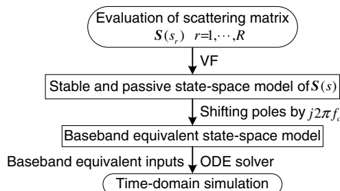
Fig. 3. Flow chart of the proposed modeling framework for the time-domain simulation of photonic systems.
