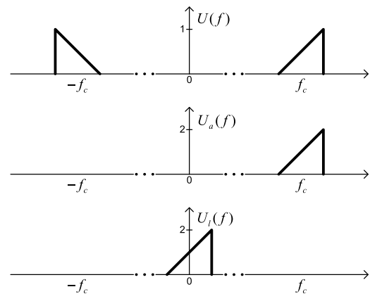
Fig. 1. Spectra of bandpass signal U(f) , analytic signal U_a(f) , and baseband equivalent signal U_l(f) .
