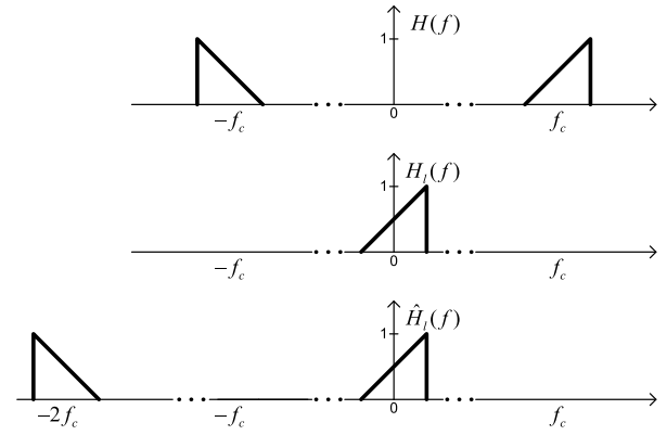
Fig. 22. Spectra of bandpass system H(f) , baseband equivalent system H_l(f) , and baseband equivalent “shifted” system \hat{H}_l(f) .
