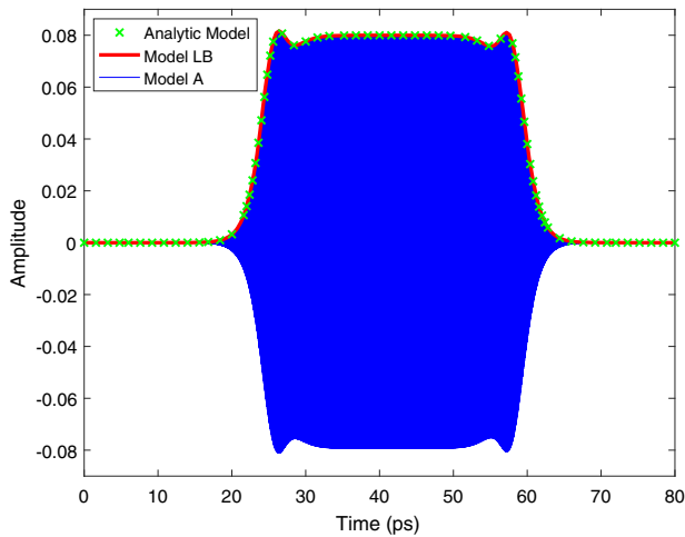
Fig. 9. Example MZI. The output at port P3 of the MZI, where the red line is the absolute value of the complex signal obtained by the time-domain simulation of Model LB, the blue line is the corresponding signal from Model A, and the marker \times denotes the same signal from the analytic model.
