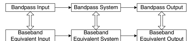
Fig. 2. Time-domain simulation of the bandpass system and baseband equivalent system.
