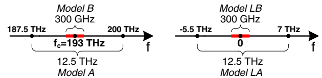
Fig. 4. Frequency ranges of Models A, LA, B, and LB.
