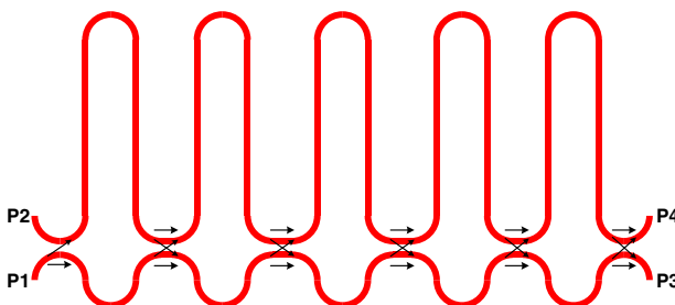
Fig. 18. Example LF. The geometric structure of the MZI lattice filter.
