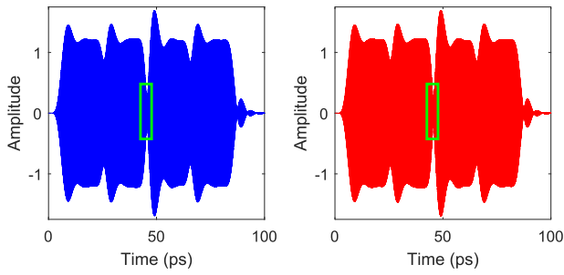
Fig. 16. Example RR. The output at port P4 of the double ring resonator. Left: the output of Model A. Right: the recovered bandpass output from Model LB.
