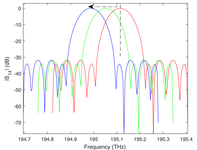
Fig. 20. Example LF. Shift of the center frequency of the passband of the lattice filter due to the tolerances of the manufacturing process.
