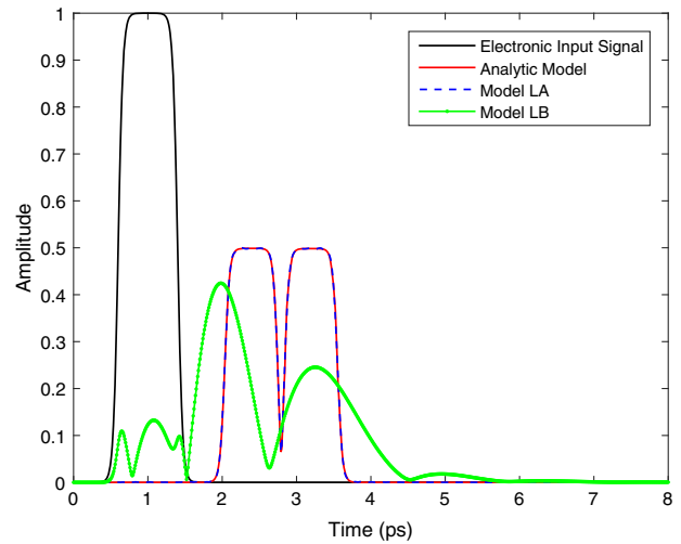
Fig. 10. Example MZI. Time-domain simulation of Models LA and LB with very narrow pulse input signal. The black line is the electronic input signal, the red solid line is the output at port P3 of the analytic model, and the blue dashed line and green dotted line indicate the outputs at the same port of Models LA and LB, respectively.
