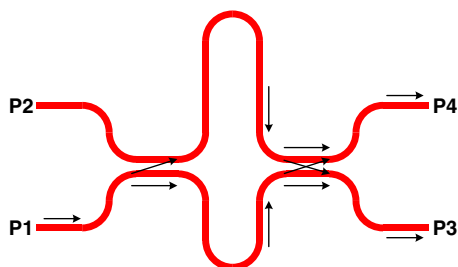
Fig. 5. Example MZI. The geometric structure of the MZI under study.
