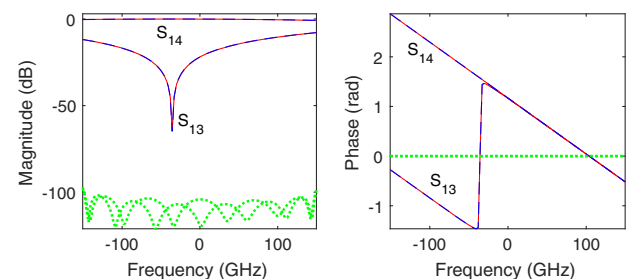
Fig. 8. Example MZI. Comparison of the magnitude (left) and phase (right) of the MZI scattering parameters extracted via Caphe (full blue line) and Model LB (red dashed line), where the green dots represent the corresponding absolute error.
