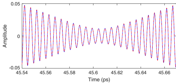
Fig. 17. Example RR. A zoom of the output at port P4 of the double ring resonator around t = 45.6 ps (the green rectangular area in Fig. 16). The blue line is used for Model A, while the red dash line is the recovered bandpass output from Model LB.
