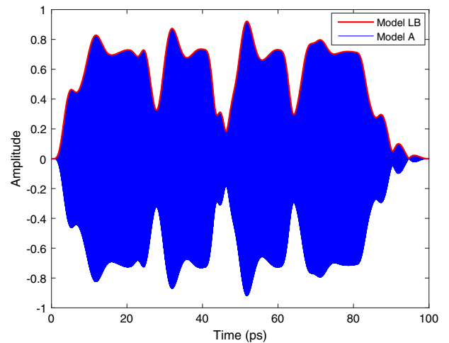
Fig. 15. Example RR. The output at port P3 of the double ring resonator, where the red line is the absolute value of the complex signal obtained by the time-domain simulation of Model LB, and the blue line is the corresponding signal from Model A.
