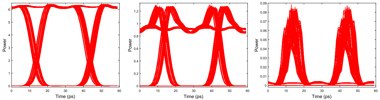
Fig. 21. Example LF. The eye diagrams at port P4 of the baseband equivalent systems of the lattice filter with passband center frequency 195.11, 195.05, and 194.98 THz (from left to right).
