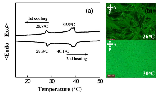
Fig. 4. (a) DSC curves of CLC-based S811 (30 wt.%) in E7 (70 wt.%) at heating/cooling rate of 1^\circ\text{C} per minute; (b) LC textures recorded under crossed polarizers for the sample at 26 ^\circ\text{C} and 30 ^\circ\text{C} .
