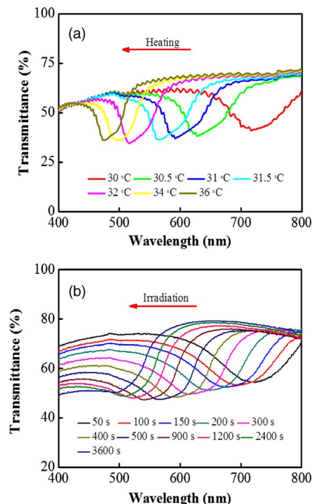
Fig. 5. Transmission spectra of CLC as functions of (a) temperature and (b) irradiation time at 850 nm.
