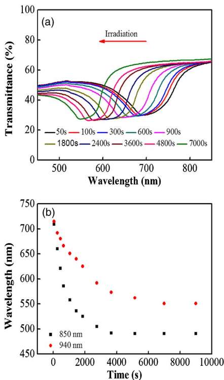
Fig. 9. (a) Transmission spectra of CLC as a function of irradiation time of 940-nm NIR. (b) Bragg wavelength as a function of NIR irradiation time. (■) 850-nm NIR irradiation on the sample; (●) 940-nm NIR irradiation on the sample.)
