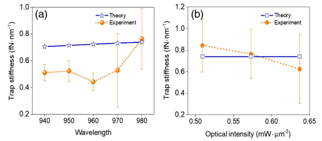
Fig. 6. (a) Trap stiffness for a single 30 nm PS sphere in a near-field trap as a function of wavelength. The experiment was done for an incident laser intensity of 0.57 \text{ mW}/\mu\text{m}^2 . The presented theoretical calculation and experimental observations were normalized to 1 \text{ mW}/\mu\text{m}^2 laser intensity. Stars, theory; solid circles, experiment; (b) trap stiffness as a function of laser intensity for an incident trapping wavelength of 980 \text{ nm} . Squares, theory; polygons, experiment.
