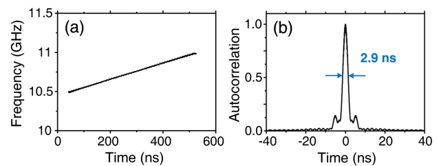
Fig. 5. (a) Recovered instantaneous frequency of LFM signal increased from 10.5 to 11 GHz in 500 ns. (b) Autocorrelation of the LFM signal in (a).
