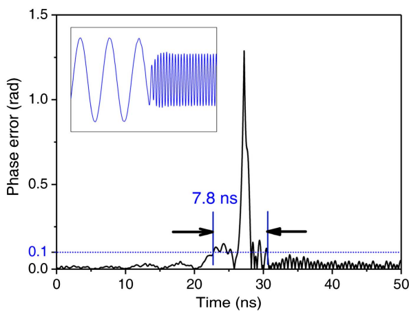
Fig. 3. Phase error during frequency transition and settling process. Inset, waveform captured by the oscilloscope at the moment that frequencies transit and settle.
