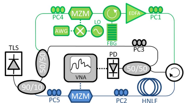
Fig. 2. Experimental setup for the demonstration of SBS-based, polarization-enhanced MWP BPFs. FBG, fiber Bragg grating.
