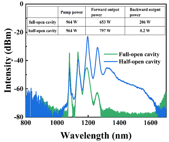
Figure 4. Compared output spectra of RFLs with a full-open cavity and a half-open cavity under the same pump power of 964 W.
