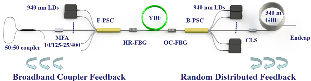
Figure 1. Experimental scheme for kilowatt-level SC generation in a single-stage RFL with a half-open cavity. MFA, mode field adapter; HR-FBG, high-reflectivity fiber Bragg grating; F-PSC, forward pump/signal combiner; YDF, ytterbium-doped fiber; OC-FBG, output coupler fiber Bragg grating; B-PSC, backward pump/signal combiner; LD, laser diode; CLS, cladding light stripper; GDF, germanium-doped fiber.
