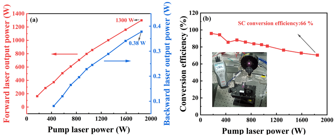
Figure 6. (a) Laser output power and (b) conversion efficiency in the RFL with a half-open cavity.
