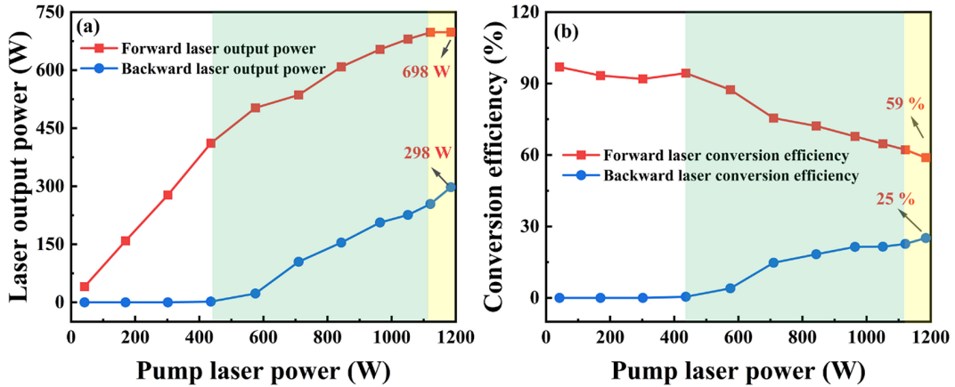
Figure 3. (a) Laser output power and (b) conversion efficiency of the RFL with a full-open cavity in both directions. The green background area is the growth area of the backward output power; the yellow background area shows that the forward output power stops increasing.
