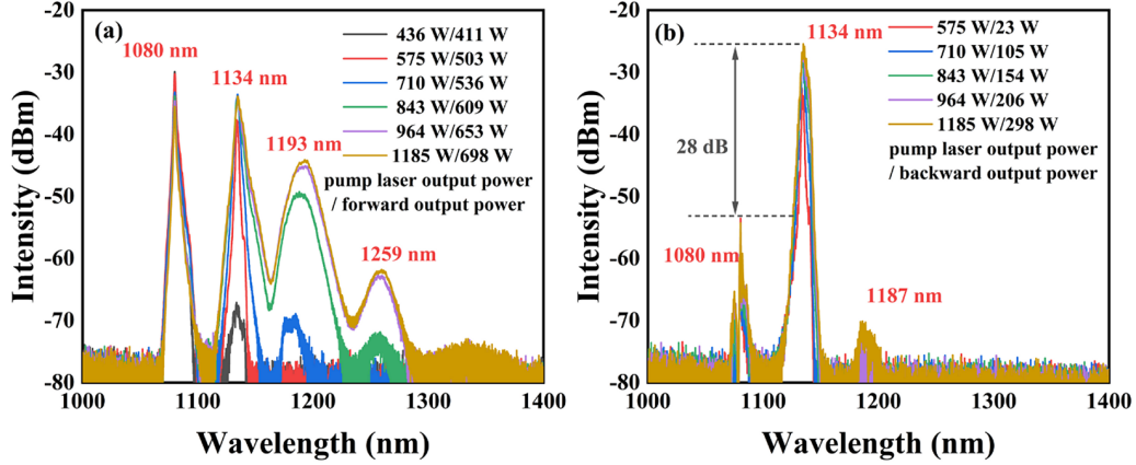
Figure 2. Output spectral evolution of pump laser power in the RFL with a full-open cavity: (a) forward direction and (b) backward direction.
