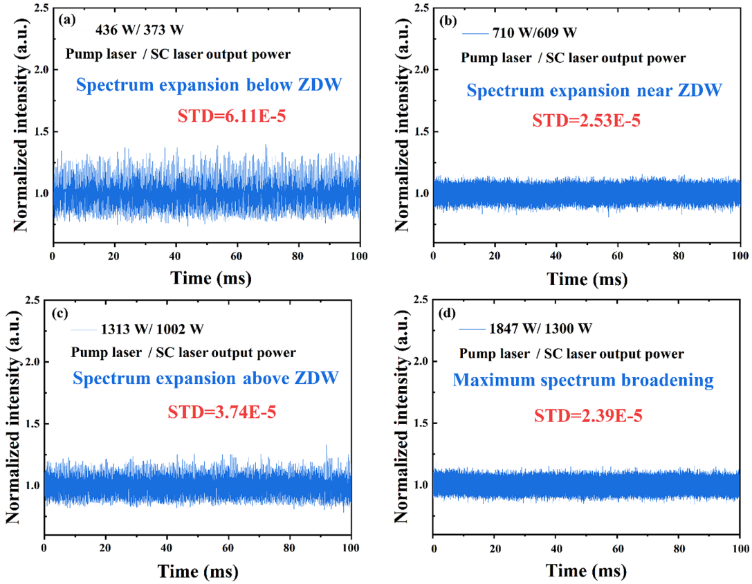
Figure 7. Normalized temporal signal of the RFL with a half-open cavity: (a) spectrum expansion below the ZDW; (b) spectrum expansion near the ZDW; (c) spectrum expansion above the ZDW; (d) maximum spectrum broadening. The recording time window is set to 100 ms.
