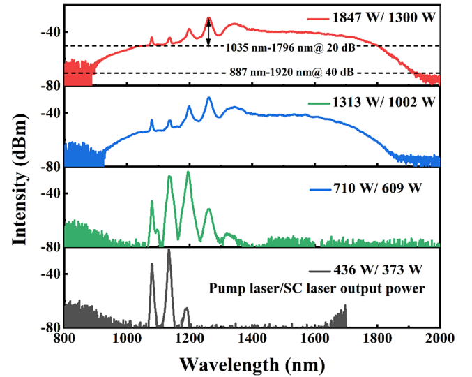
Figure 5. Output spectral evolution with pump laser power in the RFL with a half-open cavity.
