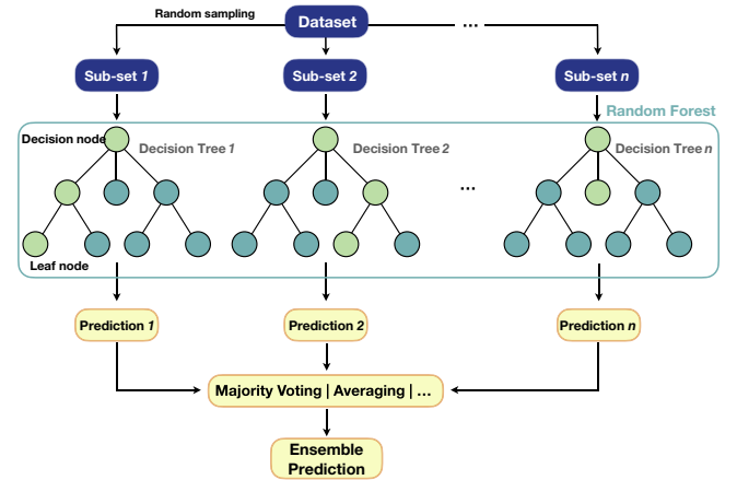
Figure 4. Sketch of a random forest, an architecture for regression or classification consisting of multiple decision trees, whose individual predictions are combined into an ensemble prediction, for example, via majority voting or averaging.
