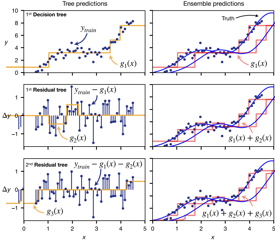
Figure 5. Example of gradient boosting with decision trees. Firstly, a decision tree g_1 is fitted to the data. In the next step, the residual difference between training data and the prediction of this tree is calculated and used to fit a second decision tree g_2 . This process is repeated n times, with each new tree g_n learning to correct only the remaining difference to the training data. Data in this example are sampled from the same function as in Figure 2 and each tree has a maximum depth of two decision layers.
