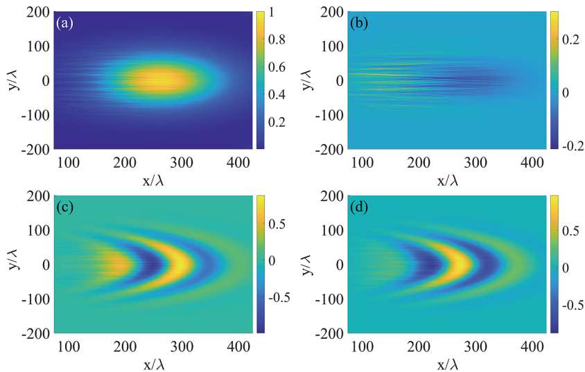
Figure 8. The spatial distributions of the Stoke parameters (a) I , (b) Q , (c) U and (d) V of the probe laser pulse at t = 650T_0 after it passes through the PDG that is induced by two intersecting laser pulses with an intersection angle \varphi . Here, all Stokes parameters are normalized to the instantaneous maximum laser intensity I_{\text{max}} . The simulation parameters are given in the text.
