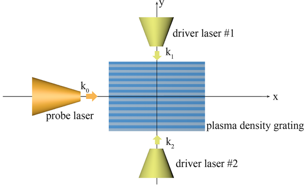
Figure 1. Schematic of laser depolarization by a PDG. The PDG driven by intersecting laser pulses #1 and #2 will be nonuniform in the y direction and also time-dependent. After the probe laser pulse passes through such a PDG, its polarization state will become nonuniform and time-dependent.
