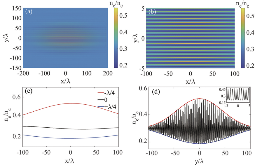
Figure 2. The electron density distribution of (a) the overall plasma region and (b) the center region [-100\lambda \leq x \leq 100\lambda] \times [-5\lambda \leq y \leq 5\lambda] at t = 590T_0 , respectively. (c) The corresponding electron density profiles along the x direction at y = -\lambda/4, 0, \lambda/4 , respectively. Here, y = \pm\lambda/4 are roughly along the plasma density trough and peak, respectively. (d) The corresponding electron density profiles along the y direction at x = 0 , in which the inset displays the enlarged density profile in the region -3\lambda < y < 3\lambda . The upper and lower envelopes of this density profile are also outlined by the red and blue curves, respectively.
