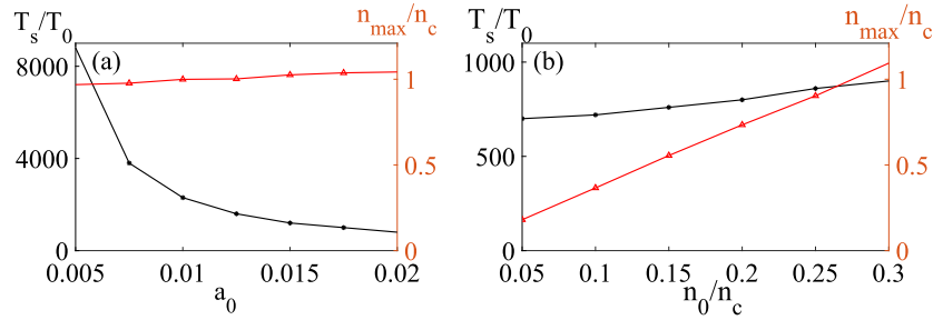
Figure 10. The saturation time T_s (black solid lines) and the maximal achievable ion density n_{\max} (red solid lines) as functions of (a) the laser intensity a_0 for a given initial plasma density n_0 = 0.3n_c and (b) the initial plasma density n_0 for a given laser intensity a_0 = 0.02 . Except for the laser intensities and initial plasma densities, other laser-plasma parameters are the same as those used in Figure 5.
