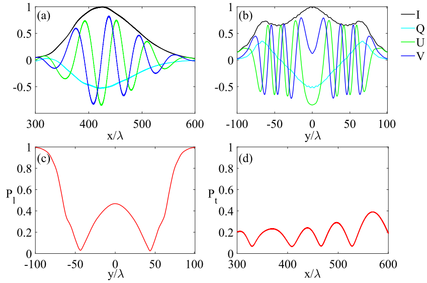
Figure 6. (a) Longitudinal profiles of the Stokes parameters at y = 0 and (b) transverse profiles of the Stokes parameters at x = 425\lambda . (c) Longitudinally averaged polarization degree P_1 and (d) transversely averaged polarization degree P_t . The simulation parameters are the same as those in Figure 5 .
