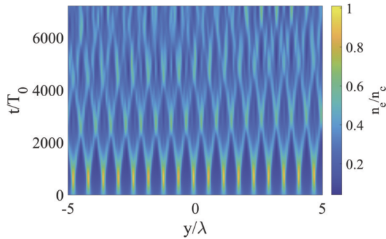
Figure 3. The time evolution of the electron density profile along the y -axis. Note that the PDG experiences a time periodic process of formation, saturation and collapse. The simulation parameters are the same as those in Figure 2.
