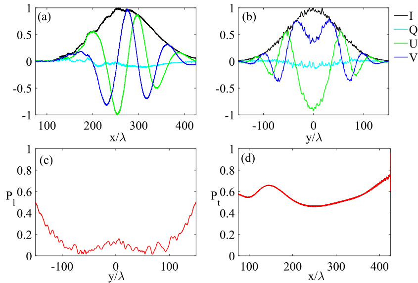
Figure 9. (a) Longitudinal profiles of the Stokes parameters at y = 0 and (b) transverse profiles of the Stokes parameters at x = 295\lambda . (c) Longitudinally averaged polarization degree P_1 and (d) transversely averaged polarization degree P_t . The simulation parameters are the same as those in Figure 8.
