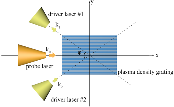
Figure 7. Laser depolarization by the PDG that is induced by two intersecting laser pulses with an intersection angle \varphi .
