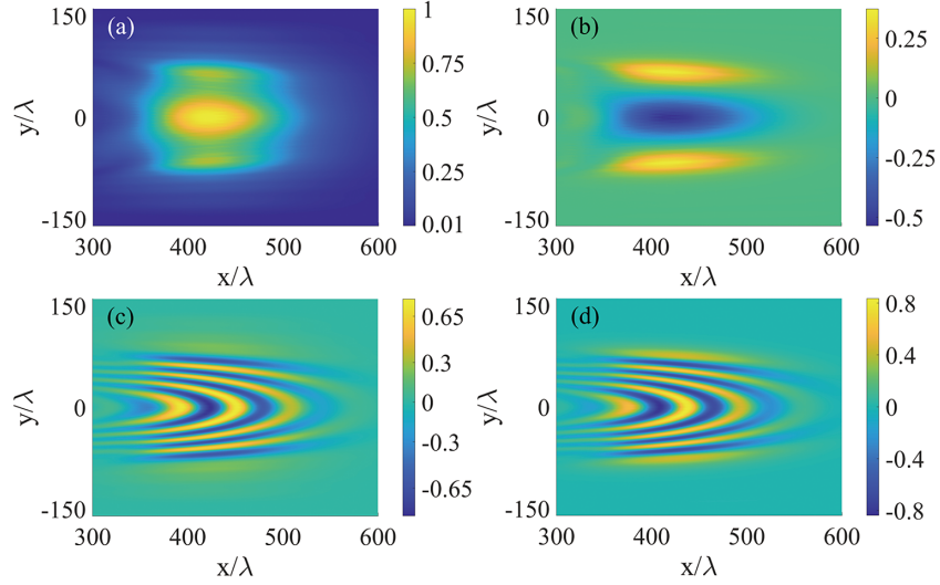
Figure 5. The spatial distributions of the Stokes parameters (a) I , (b) Q , (c) U and (d) V of the probe laser pulse at t = 940T_0 after it passes through the PDG. Here, all Stokes parameters are normalized to the instantaneous maximum laser intensity I_{\max} . The simulation parameters are given in the text.
