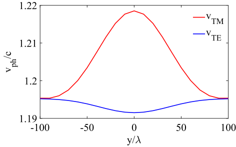
Figure 4. The phase velocities of the s-polarized ( v_{TE} ) and p-polarized ( v_{TM} ) light waves obtained from Equations (4) and (5), respectively, in which the electron density profile presented in Figure 2(d) is employed.
