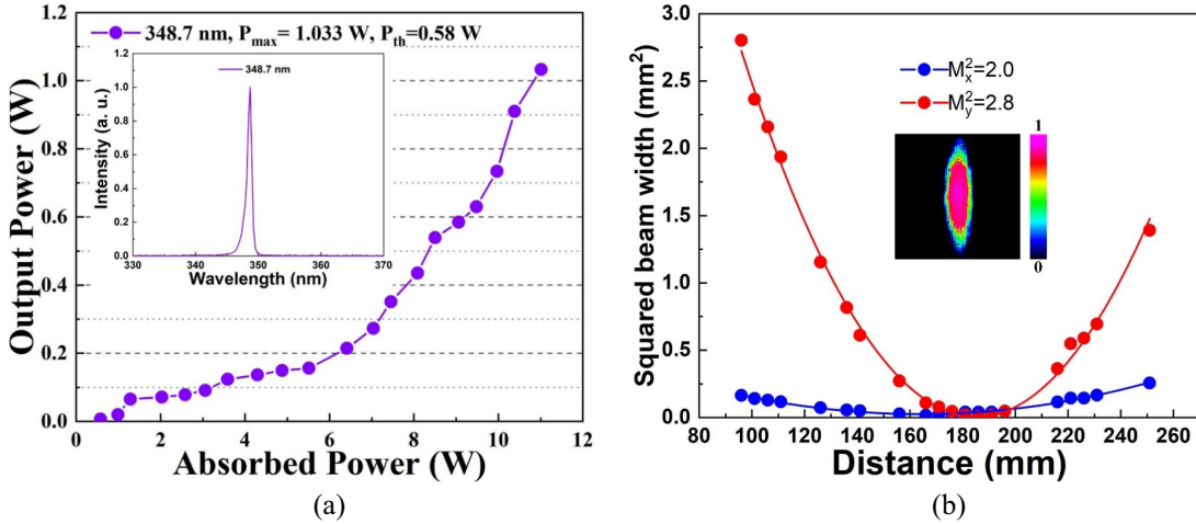
Figure 3. Output powers, laser spectrum and M^2 factors of the high-power CW single-wavelength UV laser at 348.7 nm. (a) Output powers with respect to absorbed pump powers and the laser spectrum. (b) M^2 factors of the 348.7-nm laser beam in the x and y directions.
