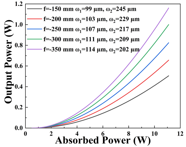
Figure 4. Simulation results of the 348.7-nm laser output powers under different effective thermal focal lengths. Here, f is the value of the effective thermal focal length and \omega_1 and \omega_2 are the laser beam sizes in the gain medium and nonlinear crystal, respectively.
