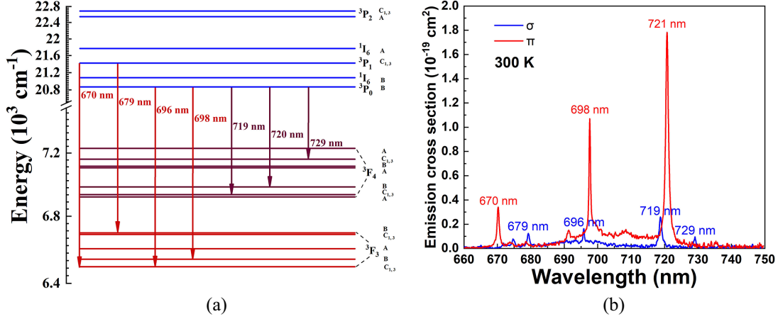
Figure 1. Some spectroscopy properties of the Pr 3+ :YLF crystal. (a) Major deep red laser transitions of the Pr 3+ :YLF crystal from {}^3P_{0,1,2} to {}^3F_4 , {}^3F_3 [38] . (b) Emission cross-sections of the Pr 3+ :YLF crystal in the deep red region.
