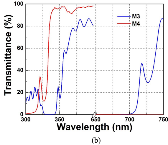
Figure 2. (a) Experimental scheme for CW UV lasers. (b) Transmittance curves of the M3 and M4 mirrors.
