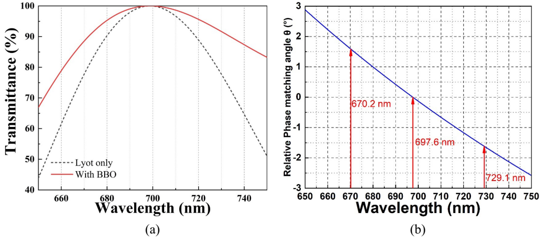
Figure 6. Simulation results to further understand the wavelength tuning. (a) Round trip TM mode transmittances comparison of using only the 1-mm thick quartz plate and both the plate and the \beta -BBO crystal at the same time. (b) Relative phase-matching angles at different wavelengths of the \beta -BBO crystal.
