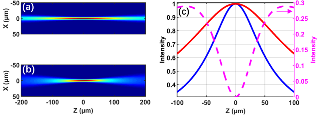
Figure 6. Intensity distributions in X - Z planes for beams without (a) and with 520 mm spatial chirp (b). (c) Intensity profiles at x = 0 in (a) and (b), red solid curve for (a), blue solid curve for (b) and purple dashed curve for the difference between them.
