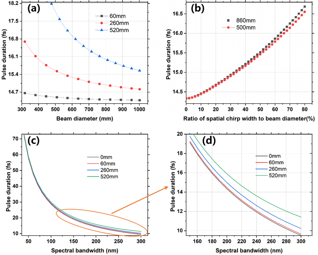
Figure 9. Curves of the pulse duration at the focal point related to (a) the beam diameter, (b) the ratio of the spatial chirp region and (c), (d) the spectral bandwidth, at different induced spatial chirp widths (0, 60, 260, 520 mm) and beam sizes (500 and 860 mm), respectively.
