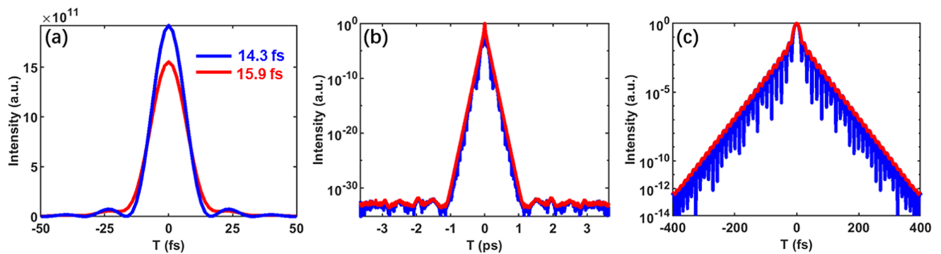
Figure 8. (a) Integrated temporal profiles in the focal plane in linear (a) and log (b), (c) scales, where the blue curve represents the ideal condition and the red curve represents the beam output from the SSGP compressor.
