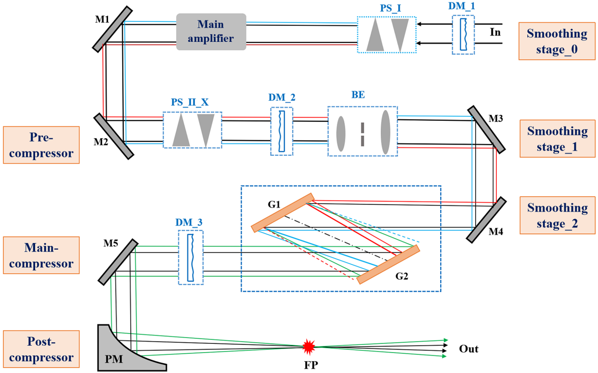
Figure 4. Optical diagrammatic sketch of the SSGP-main-compressor-based MPC. PS_I, PS_II_X: prism pair system. DM_1, DM_2, DM_3: reflective deformable mirrors with different sizes. BE: beam expander and relay imaging systems. G1, G2: diffraction gratings. M1–M5: reflective mirrors. PM: parabolic reflective mirror. FP: focal point.
