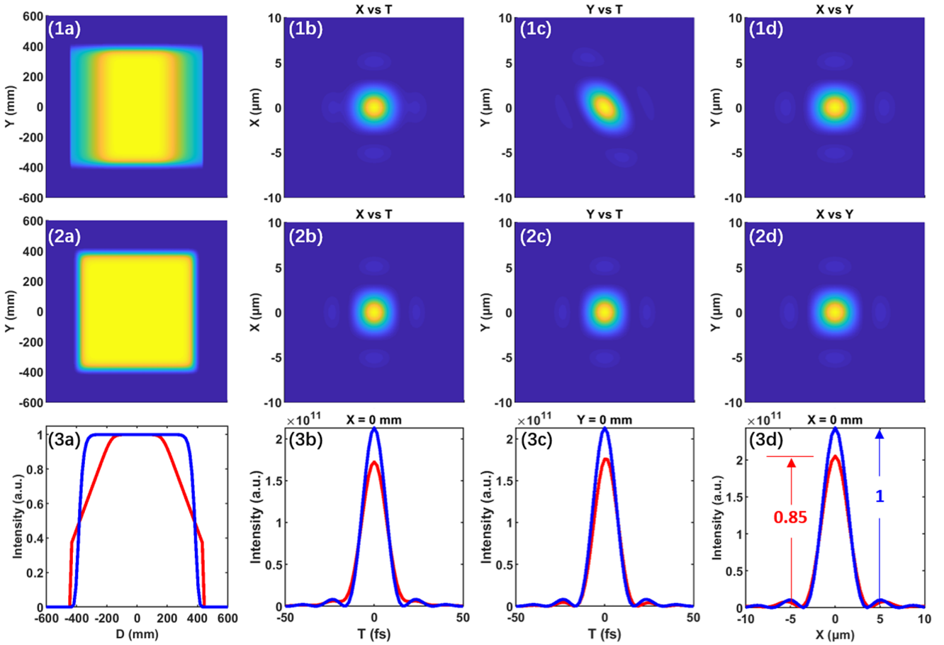
Figure 7. (1a) Near-field beam intensity without spatial chirp and spectral clipping. (1b)–(1d) Properties in the focal plane of the beam shown in (1a). (2a) Near-field beam intensity with 520 mm spatial chirp and spectral clipping. (2b)–(2d) Properties in the focal plane of the beam shown in (2a). (3a)–(3d) Intensity curves in the center along the horizontal axis of the figures above each one. The profiles in the X versus T , Y versus T and X versus Y planes are the projections in these planes of the spatiotemporal information in the focal plane.
