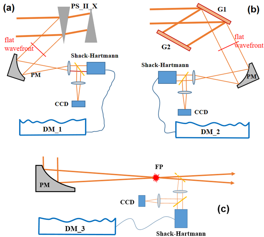
Figure 5. Optical diagrammatic sketch for the wavefront aberration measuring and controlling of (a) DM 1 , (b) DM 2 and (c) DM 3 . DM 1 , DM 2 , DM 3 : the reflective deformable mirrors corresponding to Figure 4. PM: parabolic reflective mirror.
