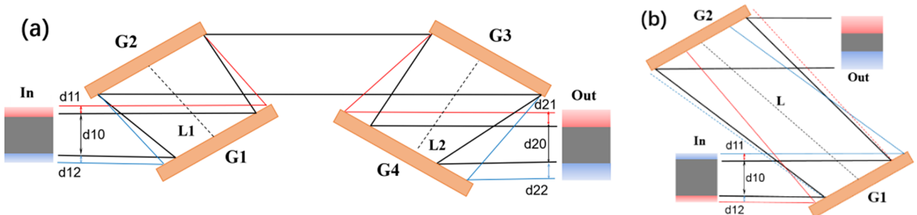
Figure 1. Optical schemes of the (a) AFGC and (b) SSGP compressor. G1–G4 are diffraction gratings; L = L_1 + L_2 . In the four beam profiles, the dark gray areas contain full spectra, and the red and blue areas contain partial longer and shorter spectra, respectively.
