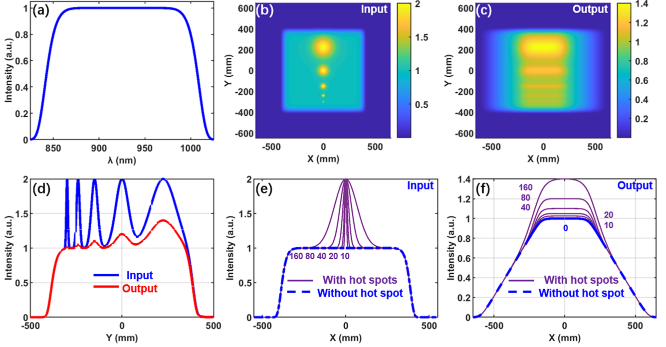
Figure 2. (a) Spectral profile. (b) Input beam with five Gaussian shape hot spots and different FWHM diameters (10, 20, 40, 80 and 160 mm, respectively). (c) Output beam from the SSGP compressor with the introduced 520 mm spatial chirp. (d) Intensity profiles at X = 0 of the input (blue curve) and output (red curve) beams in (b) and (c), respectively. (e) Intensity profiles without (dash blue curve) and with (solid purple curves) hot spots along the horizontal direction across the five peak points in (b). (f) Intensity profiles without (dash blue curve) and with (solid purple curves) hot spots along the horizontal direction across the five peak points in (c).
