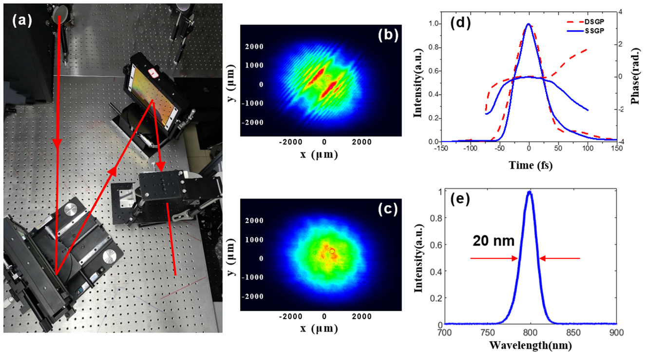
Figure 10. (a) Experimental setup of an SSGP main compressor; (b) spatial intensity modulations on the laser beam before G1; (c) output laser beam after the SSGP compressor; (d) temporal profiles at the focal point for single-pass and double-pass single-grating pairs; and (e) the spectral bandwidth of the input beam with a Gaussian profile.
