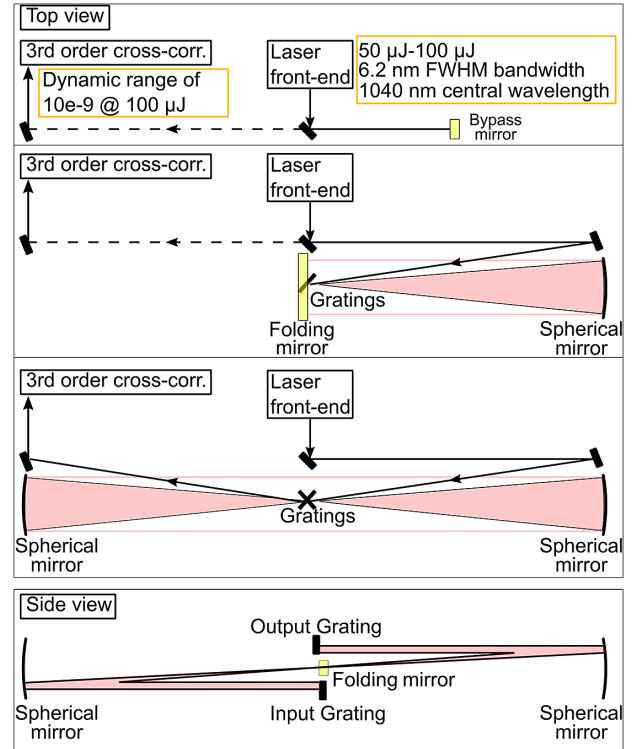
Figure 1. Schematic of the experimental stretcher setup with three configurations. First from the top, the laser pulse bypasses the stretcher using the bypass mirror; second from the top, the beam enters the stretcher, is incident on an optical grating ( G = 1740 \text{ mm}^{-1} ) and a spherical mirror ( R = 3.048 \text{ mm} ), before being reflected from a folding mirror; third from the top, the pulse enters the stretcher and transverses through an unfolded design with two gratings and two spherical mirrors. In all three configurations the beam path ends in the third-order cross-correlator (Sequoia, Amplitude) with which the temporal profile is measured. The very bottom depicts a side view of the general setup.
