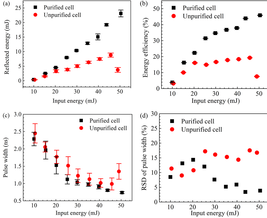
Figure 6. Comparison of SBS output parameters before and after purification of the HT270 medium at a repetition rate of 1 kHz.
