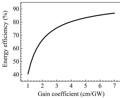
Figure 5. Calculated SBS energy efficiency with respect to the gain coefficient.
