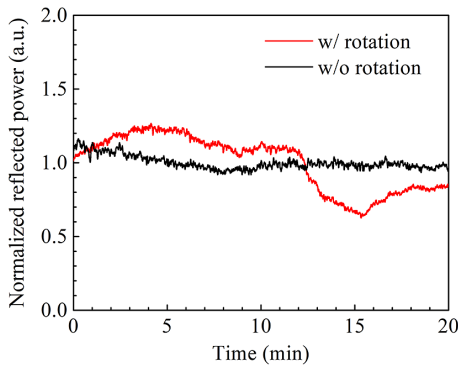
Figure 9. Stability of the SBS output energy at 2000 Hz with and without the rotating off-centered lens.
