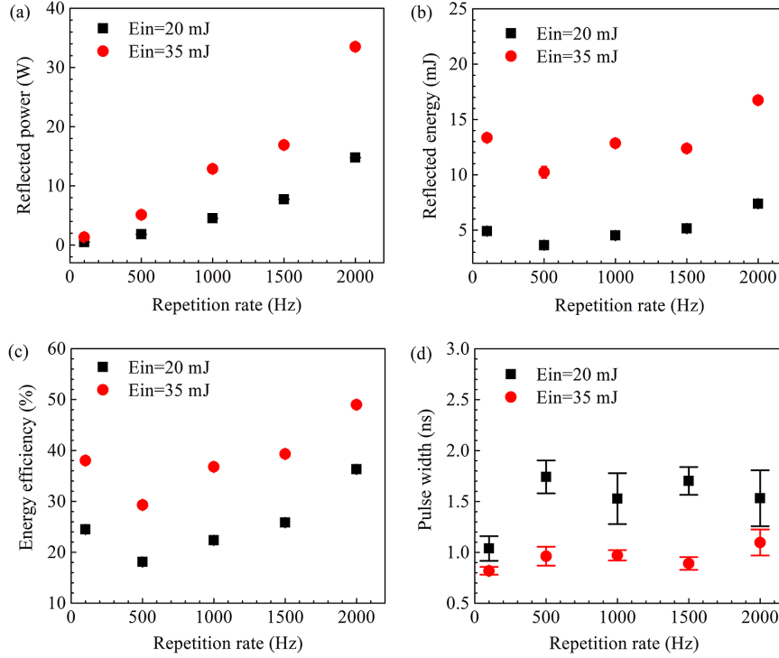
Figure 12. Measured dependences of the SBS (a) reflected power, (b) reflected energy, (c) energy efficiency and (d) compressed pulse width on the repetition rate at pump energies of 20 and 35 mJ.
