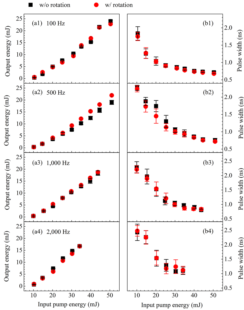
Figure 8. Measured dependences of the SBS (a1)–(a4) output energy and (b1)–(b4) compressed pulse width on the pump energy at different repetition rates with and without the rotating off-centered lens.
