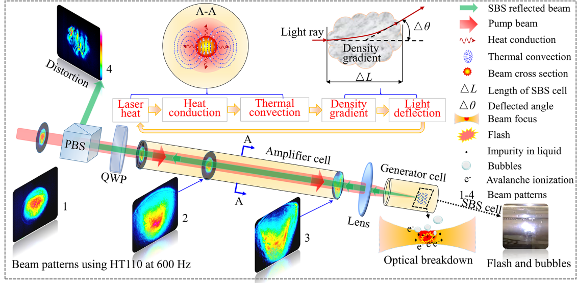
Figure 3. Schematic of thermal problems in the process of SBS pulse compression.
