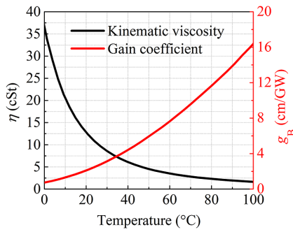
Figure 4. Kinematic viscosity of the HT270 medium and the calculated gain coefficient with respect to the temperature.
