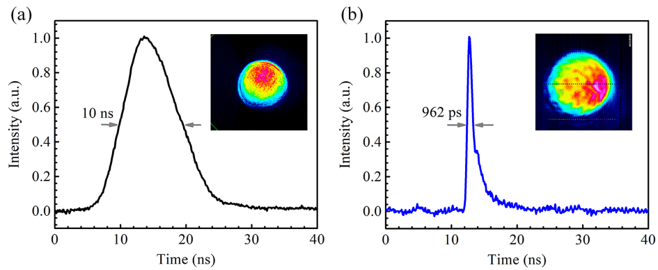
Figure 13. Waveforms and beam patterns of (a) the pump and (b) SBS compressed pulse at a pump power of 70 W.
