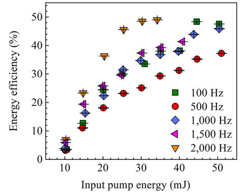
Figure 11. Measured dependence of the SBS energy efficiency on the pump energy at different repetition rates.
