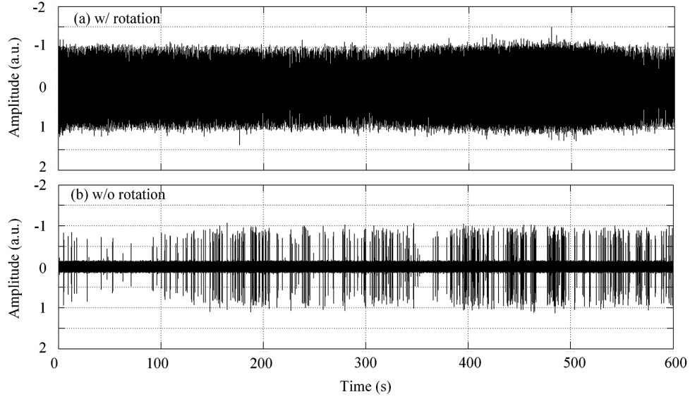
Figure 10. Audio amplitude of the SBS output (a) with and (b) without the rotating off-centered lens at 2000 Hz.
