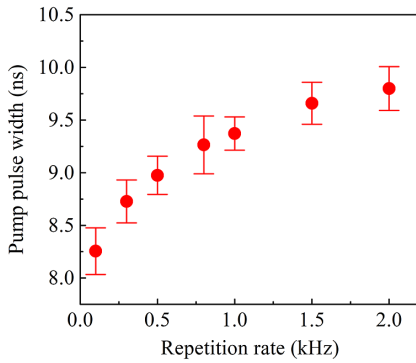
Figure 2. Pump pulse widths of the laser system with different repetition rates.
