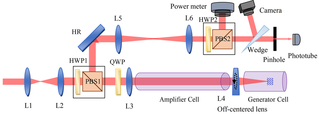
Figure 1. Schematic of the experimental setup for SBS pulse compression based on a rotating off-centered lens (HWP1 and HWP2, half-wave plates; L1–L6, lenses).
