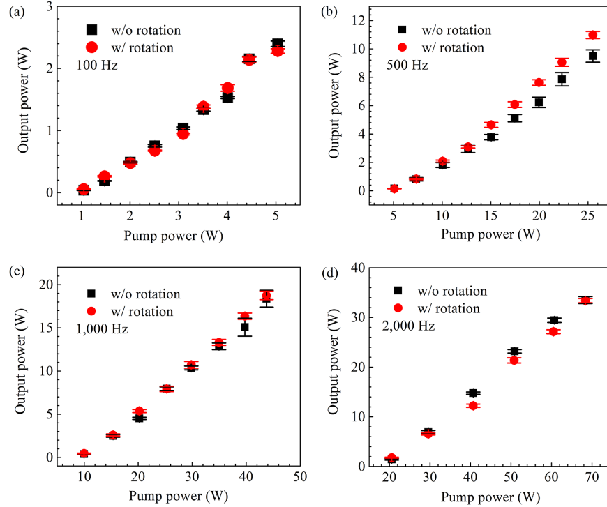
Figure 7. Measured dependence of the SBS output power on the pump power at repetition rates of (a) 100 Hz, (b) 500 Hz, (c) 1000 Hz and (d) 2000 Hz with and without the rotating off-centered lens.
