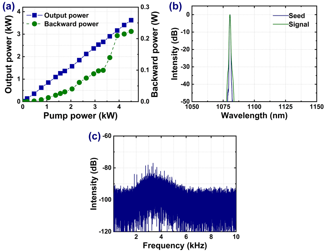
Figure 3. Basic output properties of the fiber amplifier employing the backward pumping scheme: (a) power curve; (b) output spectrum at the maximum output power; (c) Fourier spectrum of the signal laser at the maximum output power.
