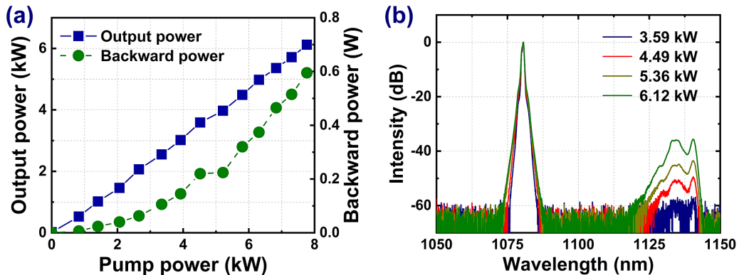
Figure 4. Basic output properties of the fiber amplifier employing the bidirectional pumping scheme: (a) power curve; (b) output spectra.
