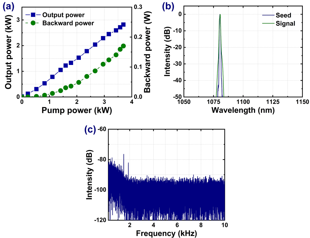
Figure 2. Basic output properties of the fiber amplifier employing the forward pumping scheme: (a) power curve; (b) output spectrum at the maximum output power; (c) Fourier spectrum of the signal laser at the maximum output power.
