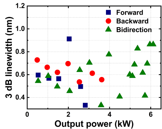
Figure 6. The 3 dB spectral linewidths of the signal laser at different output powers.
