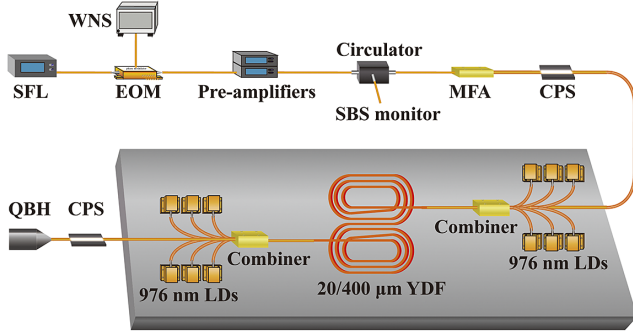
Figure 1. Experimental setup of the all-fiberized and narrow-linewidth fiber amplifier.
