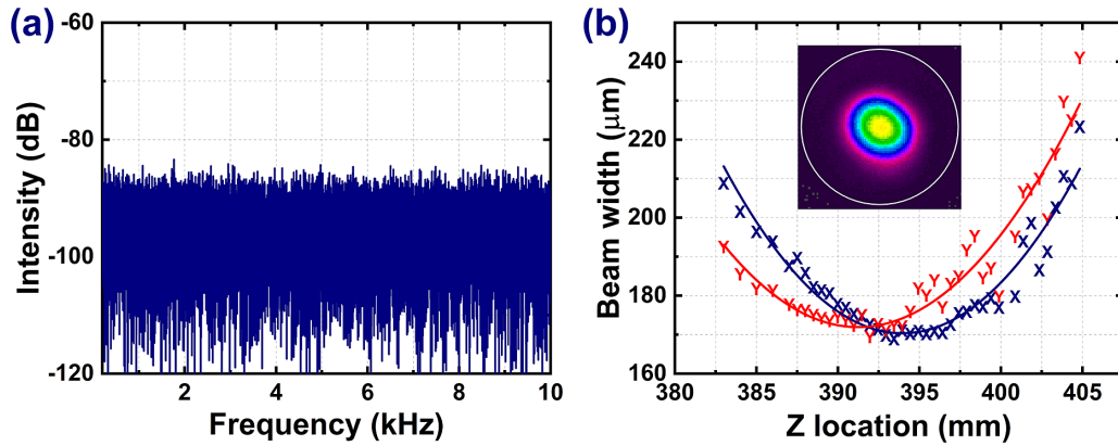
Figure 5. Output properties of the signal laser at the maximum output power in the fiber amplifier employing the bidirectional pumping scheme: (a) Fourier spectrum; (b) beam quality factor (the insert figure is beam profile at the location of Z = 393.5 mm).
