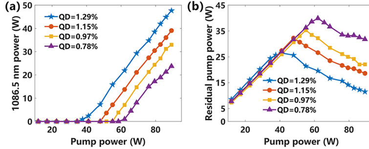
Figure 6. Power evolutions of (a) the 1086.5 nm signal and (b) the residual pump as functions of pump power, with different QD outputs.
