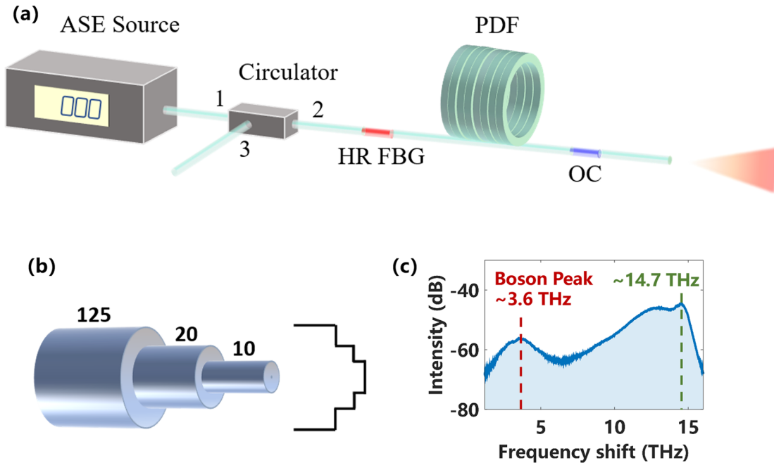
Figure 1. (a) The experimental setup of the low-QD RFL. (b) The structure of the PDF. (c) Properties of the Raman frequency shift of the PDF.
