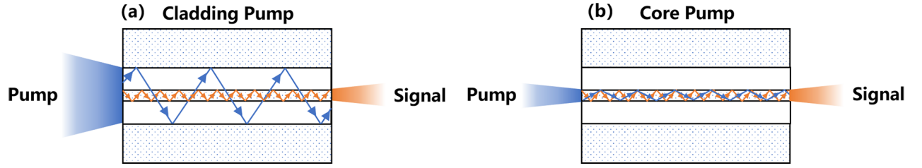
Figure 2. Schematic diagrams of laser transmission in (a) cladding pumping and (b) core pumping.
