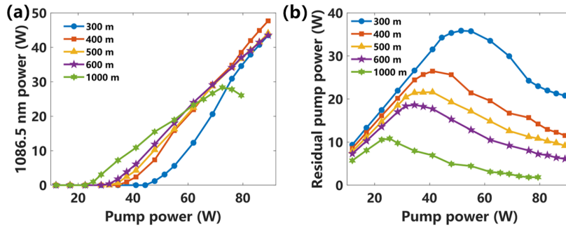
Figure 5. Power evolutions of (a) the 1086.5 nm signal and (b) the residual pump as functions of pump power, with different PDF lengths.
