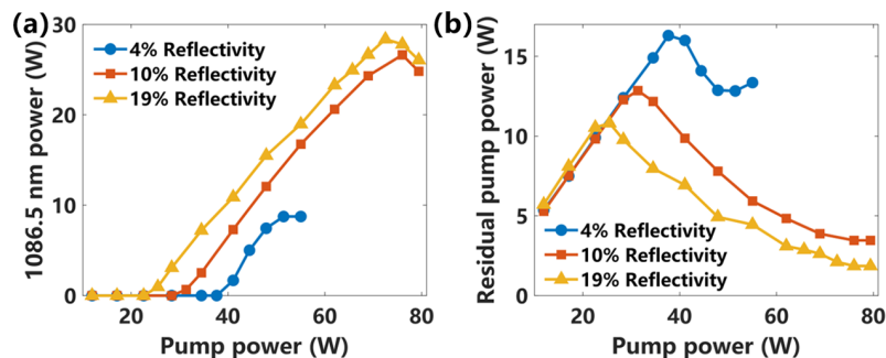
Figure 4. Power evolutions of (a) the 1086.5 nm signal and (b) the residual pump as functions of pump power, with different OC reflectivities.
