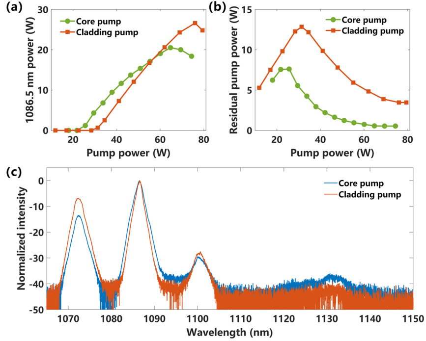
Figure 3. Power evolutions of (a) the 1086.5 nm signal and (b) the residual pump, in two pump schemes. (c) The normalized intensity spectra as a function of wavelength, with 55 W pump power.
