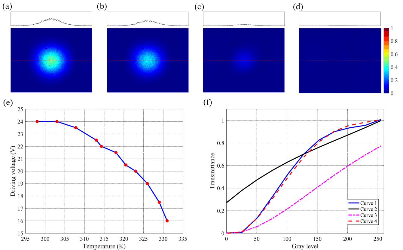
Figure 9. (a) Distribution of light field after transmittance and temperature increase at 24 V. (b)–(d) Light field distribution at 22 V, 20 V and 19 V, respectively. (e) OASLM driving voltage as a function of temperature, where red data points represent experimental data. (f) Gamma curves under different driving conditions and different temperatures. Curve 1: 298 K, 24 V, 600 mA; curve 2: 326 K, 24 V, 600 mA; curve 3: 326 K, 19 V, 600 mA; curve 4: 326 K, 19 V, 1000 mA.
