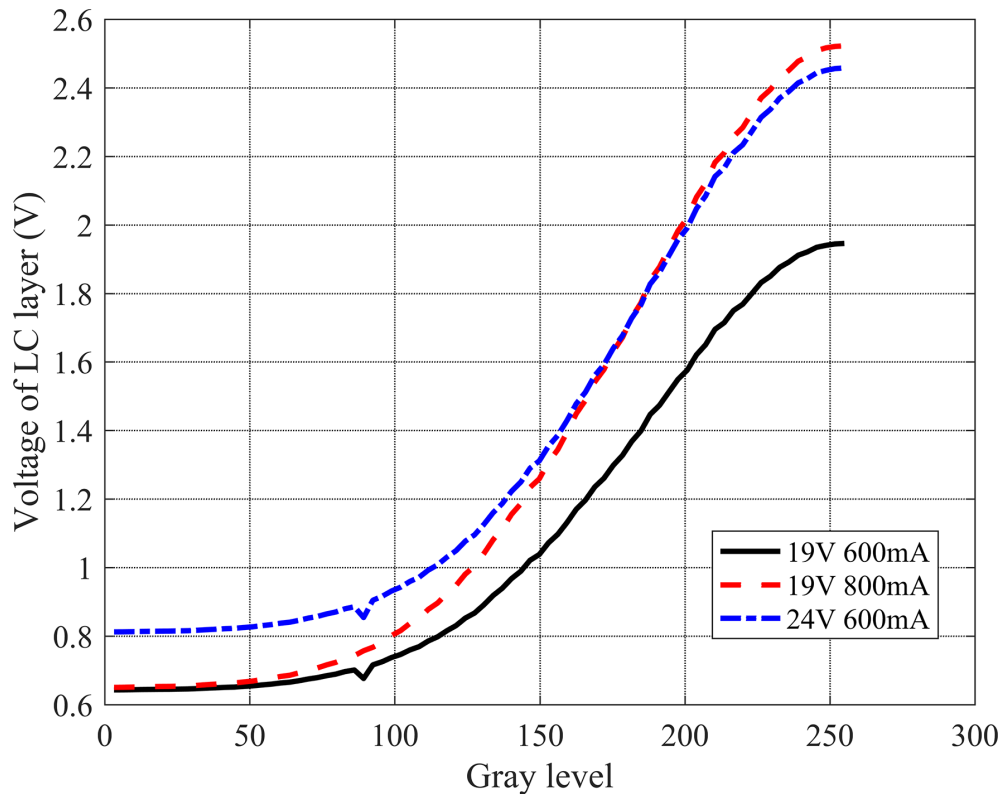
Figure 5. Voltage of liquid crystal layer changes with the loaded gray level under different driving conditions.
