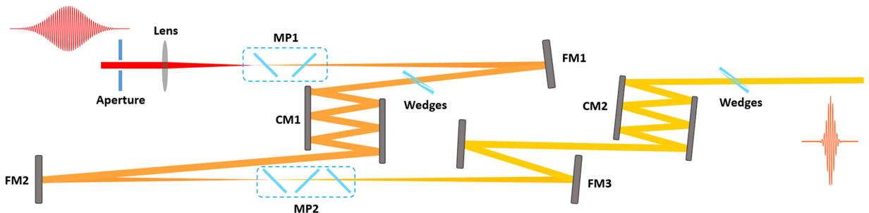
Figure 1. Schematic view of the multi-plate (MP) setup with two compression stages (FM, focusing mirror; CM, chirped mirror). For single-stage operation, the beam parameters are measured after the first pair of chirped mirrors CM1 and before the refocusing mirror FM2.
