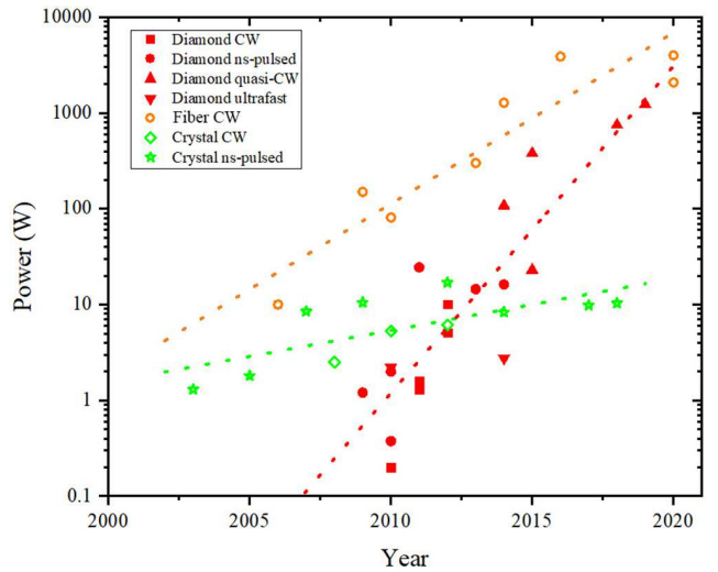
Figure 1. Achieved output power of DRLs [8,23,28–43] compared with other crystalline Raman lasers [33,44–53] and Raman fiber lasers [54–61] .
