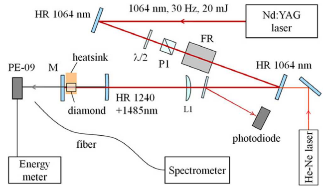
Figure 3. Schematic of the external cavity Raman laser [67] .
