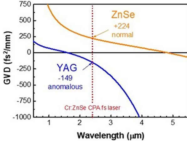
Figure 2. Dispersion curves of YAG and ZnSe versus wavelength. The dotted line shows the pump wavelength of 2.4 \mu\text{m} .
