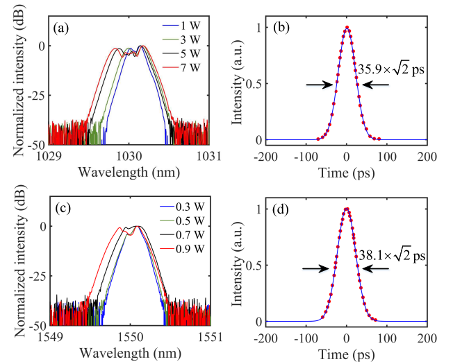
Figure 2. Experimental characterization of output pulses from (a), (b) pump and (c), (d) signal after two-stage fiber amplifiers, including (a), (c) the measured optical spectra and (b), (d) corresponding auto-correlation traces. Note that the traces given in (b) and (d) were measured at the average power of 7 and 0.9 W, respectively. The actual intensity profiles are scaled down by a factor of \sqrt{2} under an assumption of Gaussian pulses.
