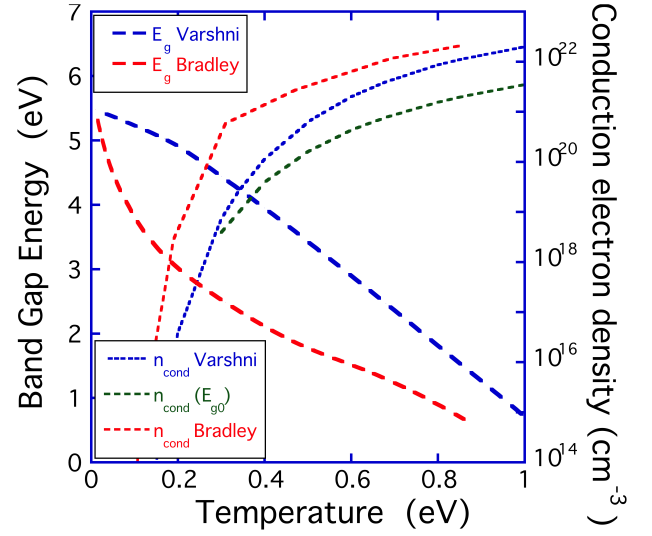
Figure 9. Energy gap versus temperature and electron density in the conduction band calculated using the formula from Varshni (constant density, effect of temperature only) and that from Bradley et al. (along the Hugoniot). In this last case, the temperature has been related to compression through SESAME table 7834. For comparison we also show the case in which there is no variation of density and variation of energy gap (i.e., the increase in temperature only affects the Fermi–Dirac distribution of electrons).
