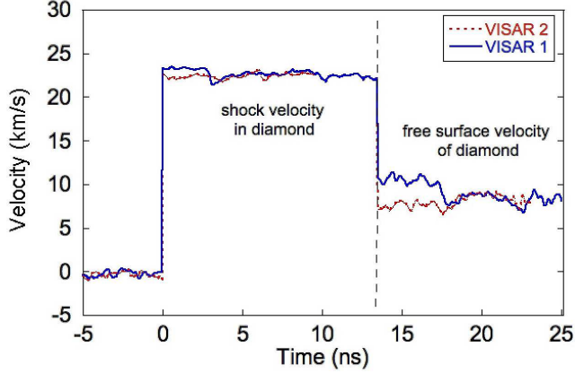
Figure 4. Time history of the shock velocity in diamond obtained by analyzing the fringe shift of the two VISARs from shot 15 (Figure 3). Here t = 0 is the time of shock breakout at the inner nickel/diamond interface and the shock breakout at diamond rear side takes place 13.48 ns afterwards. The first part of the graph represents the shock velocity in diamond. The second part shows the free surface velocity of diamond after shock breakout at the target rear side.
