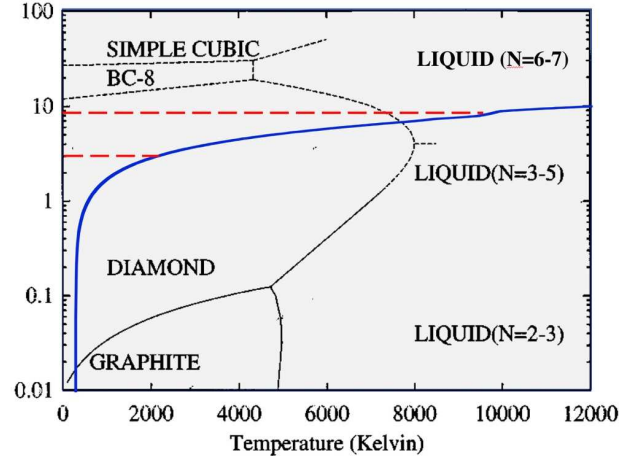
Figure 7. Phase diagram of carbon according to Grumbach and Martin [7] and shock Hugoniot from the SESAME table 7834. The two dashed horizontal red lines show the range of pressures reached in diamond in our shot 15.
