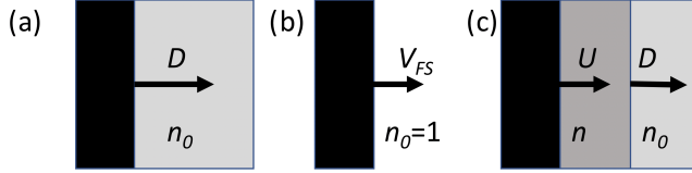
Figure 2. Reflection of the VISAR probe beam: (a) from a reflecting shock traveling in the material; (b) from a free surface travelling in vacuum; (c) from a reflecting surface embedded in a compressed transparent material.
