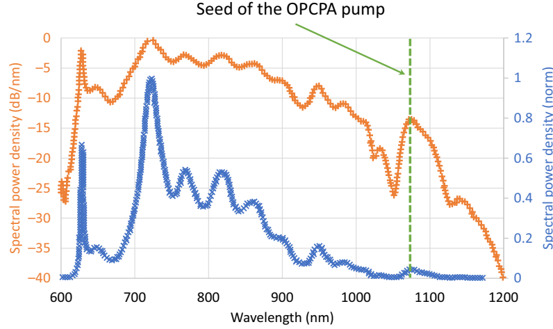
Figure 2. Vention oscillator spectrum.
