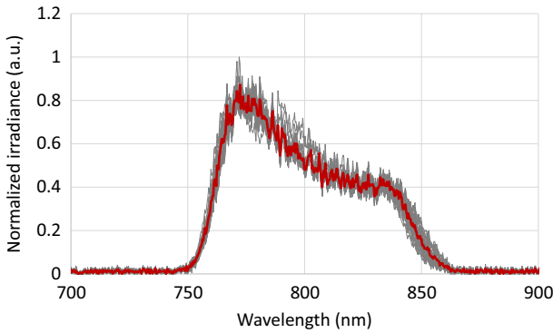
Figure 7. Stability of the OPCA spectrum over 7 h continuous operation. The red curve is the average of the data acquired at 10 min intervals that we represented by the gray curves.
