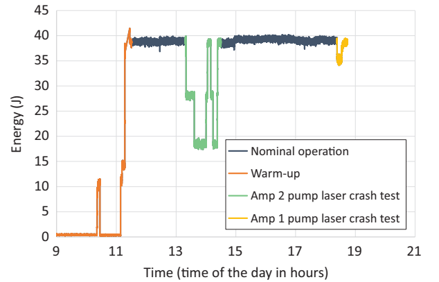
Figure 20. Long-term stability test for the 1 PW level amplifier during 1 day of operation showing the energy of all the shots before compression.
