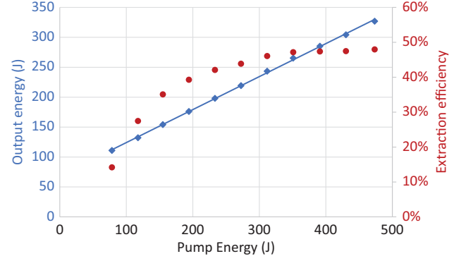
Figure 16. Extraction efficiency for the 10 PW level amplifier AMP3.2.
