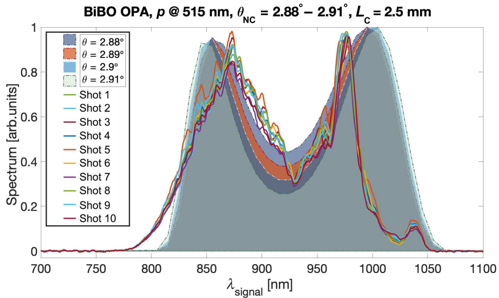
Figure 8. Experimental results for the BiBO OPA stage: amplified spectrum for a 2.5 mm crystal. Different noncollinear angles are plotted to show the influence of \theta_{NC} on the spectral dip around 920 nm.
