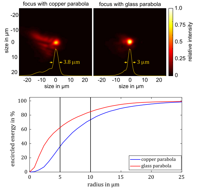
Figure 2. Comparison of the focal spot of the copper and glass parabolas, taken during alignment mode inside the target chamber, showing the improvement introduced by the new optic (upper half). The yellow curve corresponds to a lineout over the horizontal direction through the centre, which additionally shows the FWHM of the foci. The lower part of the figure shows the comparison of the encircled energy for both parabolas.
