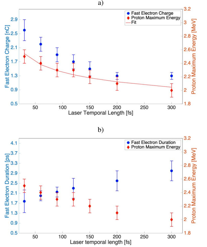
Figure 3. Simultaneous detection of the (a) ultrafast electron charge, (b) temporal length, and maximum proton energy for different laser durations.
