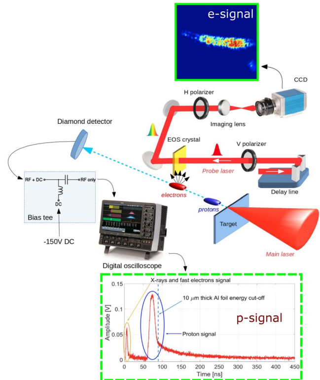
Figure 1. Experimental setup. The FLAME laser is sent to an aluminium target. The charged particles emitted during this interaction are revealed by two single-shot time resolved measurements: electro-optic sampling diagnostics, able to measure the electric field carried by relativistic fast electrons, and a time-of-flight diamond detector, used to measure the temporal distribution of protons arriving at it and to retrieve their energy spectra [20] .
