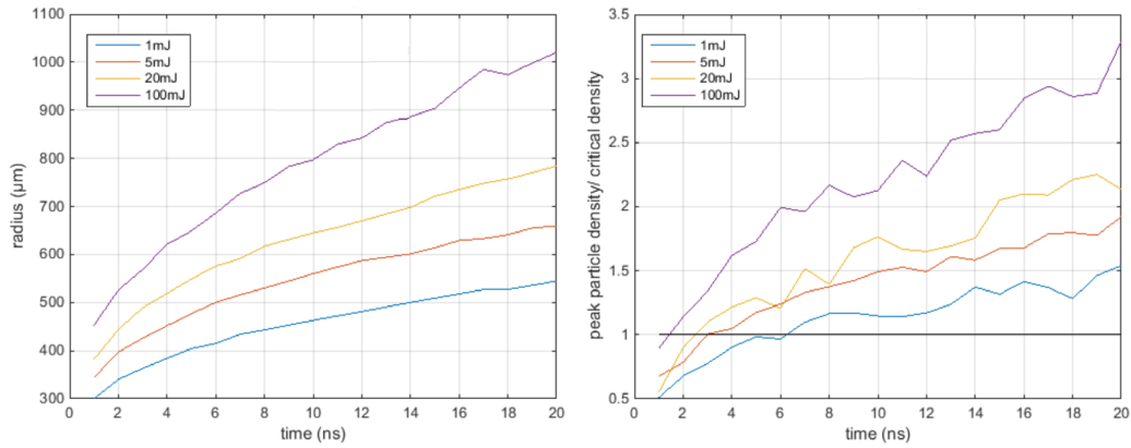
Figure 7. The blast wave radii (left) and the corresponding ratio of the peak electron density to the critical density (right). Time evolution up to 20 ns for 1, 5, 20 and 100 mJ absorbed energy deposited at z = 0.1 cm prior to the centre of the throat. Initial density was set to n = 3.39 \times 10^{18} \text{ cm}^{-3} .
