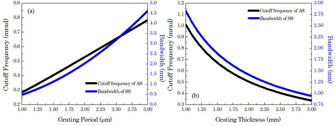
Figure 3. Dependence of the Bragg selectivity on the grating period and thickness: (a) \lambda_0 = 1053 nm, d = 2.5 mm, \phi = 90^\circ ; (b) \lambda_0 = 1053 nm, \Lambda = 1.5 μm, \phi = 90^\circ .
