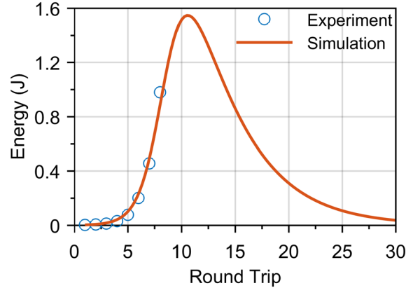
Figure 5. Energy output versus the number of round trips. The blue circles and the red curve correspond to the experimental and simulation results, respectively.
