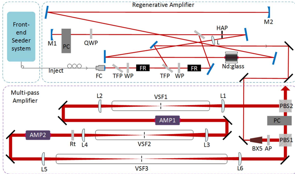
Figure 1. Schematic of the regenerative amplifier and multi-pass amplifier. FC, fiber beam collimator; TFP, thin-film polarizer; WP, half-wave plate; QWP, quarter-wave plate; FR, Faraday rotator; M1, M2, cavity concave mirrors; PC, Pockels cell; AMP, laser head with a diode-pumped Nd:glass rod in the center surrounded by laser diode bars; L, biconvex lens; HAP, hard aperture; BX5, 5 \times beam expander; AP, 8.1 mm \times 8.1 mm square soft edge aperture; PBS, polarization beam splitter; L1–L6, plane-convex lenses; VSF1–VSF3, vacuum spatial filters; AMP1, AMP2, two identical laser heads with Nd:glass rod in center surrounded by four xenon lamps.
