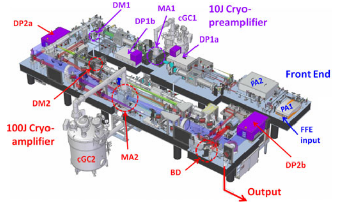
Figure 2. 3D model of DiPOLE100X: FFE = fibre front end, DP = diode pumps, cGC = cryogenic gas coolers, DM = deformable mirrors, BD = beam diverter, FFE = fibre front end (not shown).
