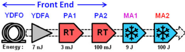
Figure 1. Schematic of DiPOLE100X amplifier chain, showing typical output energy at each amplifier stage: YDFO = Yb-silica fibre oscillator; YDFA = Yb-silica fibre amplifier (inc. temporal pulse shaping); PA = room-temperature preamplifier (1 = Yb:CaF 2 regenerative, 2 = Yb:YAG multi-pass); MA = main cryogenic amplifier (ceramic Yb:YAG multi-slab).
