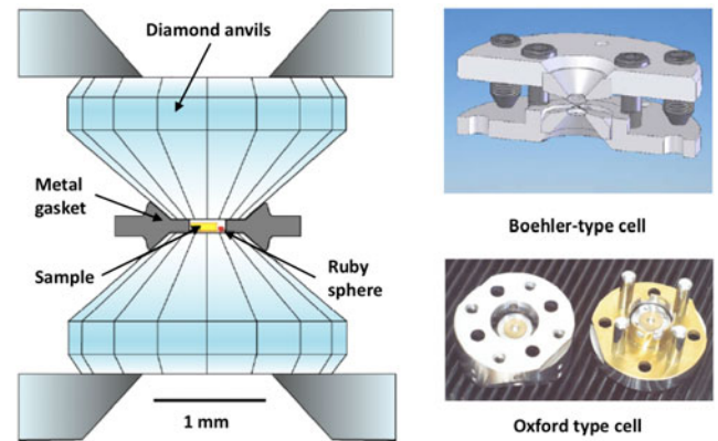
Figure 3. Schematic of a typical DAC setup including the diamond anvils, metal gasket, sample and a ruby sphere pressure reference. The figure also includes some examples of different cell/gear box systems used.
