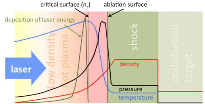
Figure 2. Diagram of interaction between a solid/liquid target and a laser showing ablation of the surface material. The laser light can only propagate through the plasma up to the critical density n_c at the critical surface, where it is reflected. The highest temperature is found at the critical surface. The temperature then drops between the critical surface and the solid target. Heat from the critical surface is conducted down the temperature gradient towards the solid surface, where it generates more plasma, keeping the ablation process going. The cooling process due to the rapid expansion is balanced by laser energy deposition keeping the temperature of the low density corona roughly constant. The region between the ablation and critical surfaces is often referred to as conduction zone.
