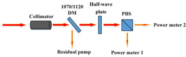
Figure 7. The measurement setup of PER.
