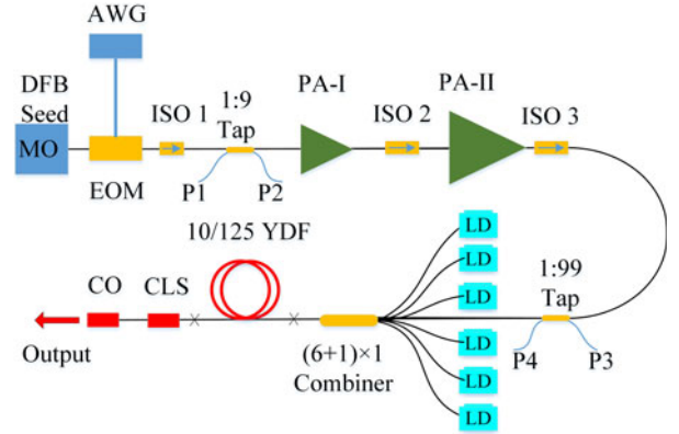
Figure 1. Experimental setup of monolithic fiber amplifier system (MO: master oscillator; PA, pre-amplifier; CO, collimator).
