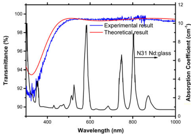
Figure 2. Transmission spectra of ultra-BAC and N31 [20] Nd:glass absorption spectra (black curve).
