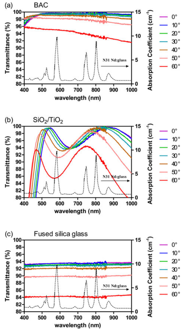
Figure 3. Variation of the transmission spectra with light incidence and N31 Nd:glass absorption spectra (black dashed curve). (a) BACs, (b) SiO 2 /TiO 2 coatings and (c) uncoated fused silica glass.
