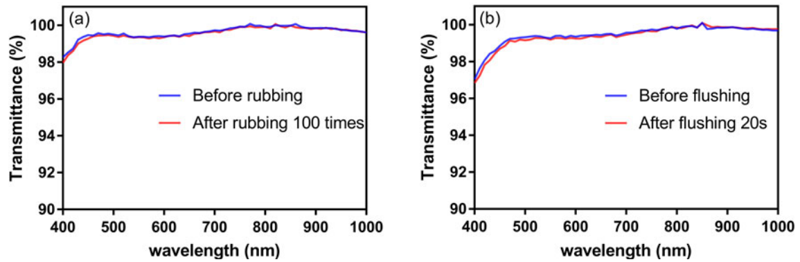
Figure 7. (a) Transmittance of the BAC before and after rubbing by the cotton ball immersed with ethanol 100 times. (b) Transmittance of the BAC before and after deionized water flushing.
