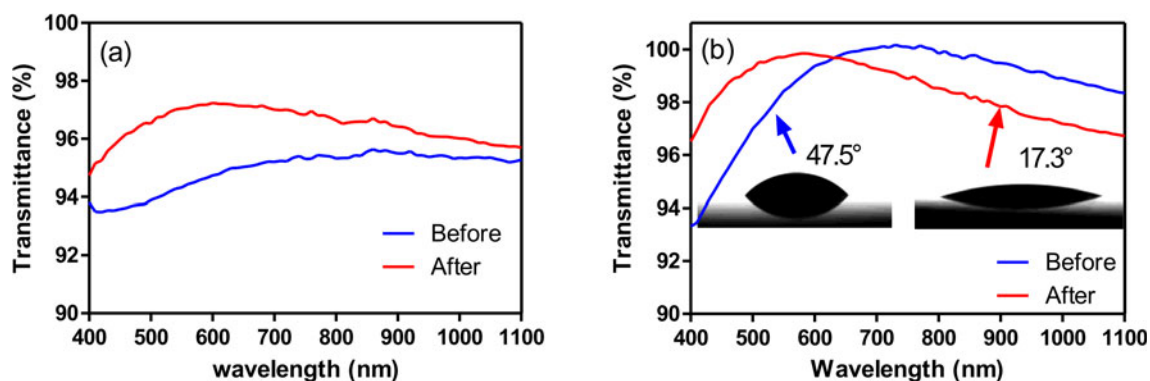
Figure 5. Transmittance of (a) BA60 and (b) LA90 before and after baking at 500 °C.
