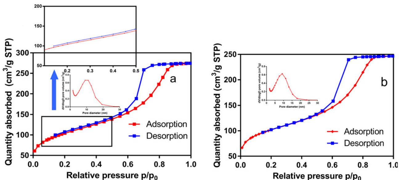
Figure 6. N 2 adsorption/desorption isotherm, and pore size distribution curve of LA90 after (a) 200 °C treatment and (b) 500 °C treatment.
