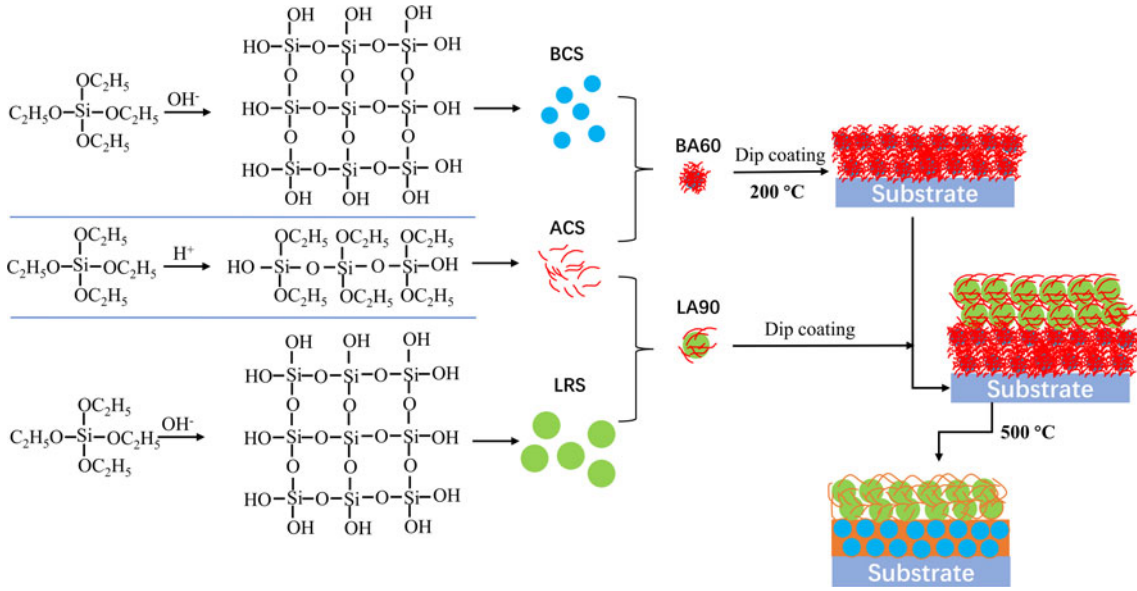
Figure 1. Preparation of ultra-BACs.
