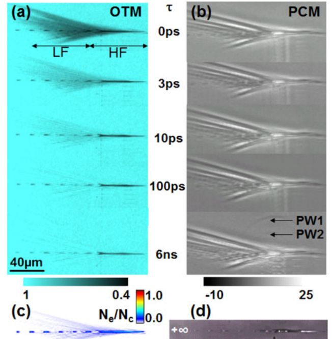
Figure 1. Time-resolved observation of laser excitation and subsequent relaxation in fused silica in (a) OTM and (b) PCM modes at energies significantly above the void-formation threshold (high-energy range). Input energy E = 43 \mu\text{J} and pulse duration t_p = 160 \text{ fs} . Two characteristic regions in terms of dynamics are indicated as LF region and HF region. (c) Estimated maximum electronic density at zero delay, at the excitation peak. (d) PCM aspect of the permanent damage. Transmission and relative phase change scale bars are given, as well as normalized (to critical density at 800 nm) scales for carrier density. The laser pulse is coming from the left.
