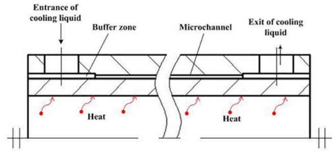
Figure 2. Schematic diagram of microchannel heat sink.
