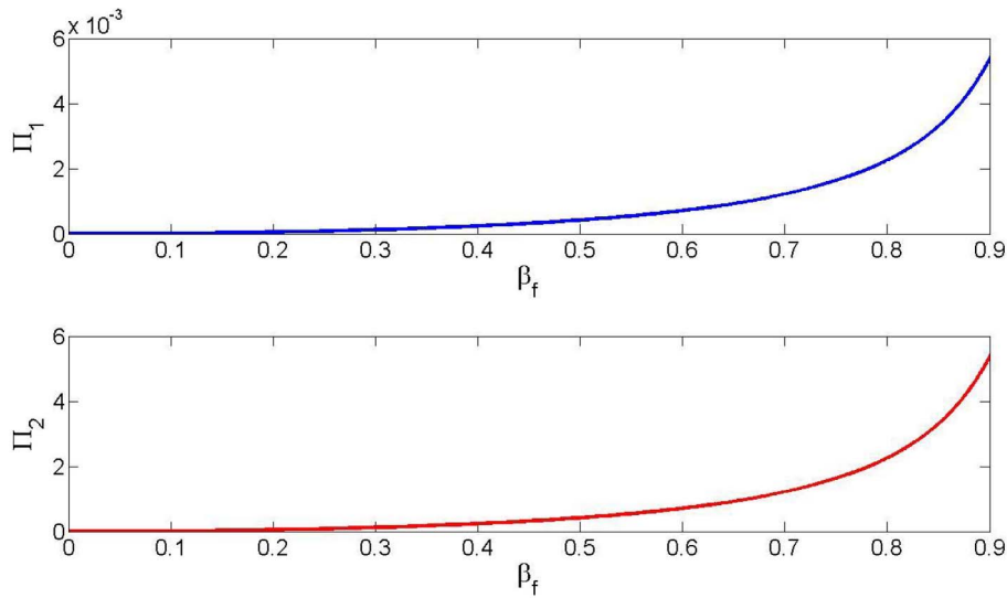
Figure 9. The pressures of the dimensionless shocked target \Pi_1 and the shocked flyer \Pi_2 for \rho_{0t}/\rho_{0f} = K = 1000 .
