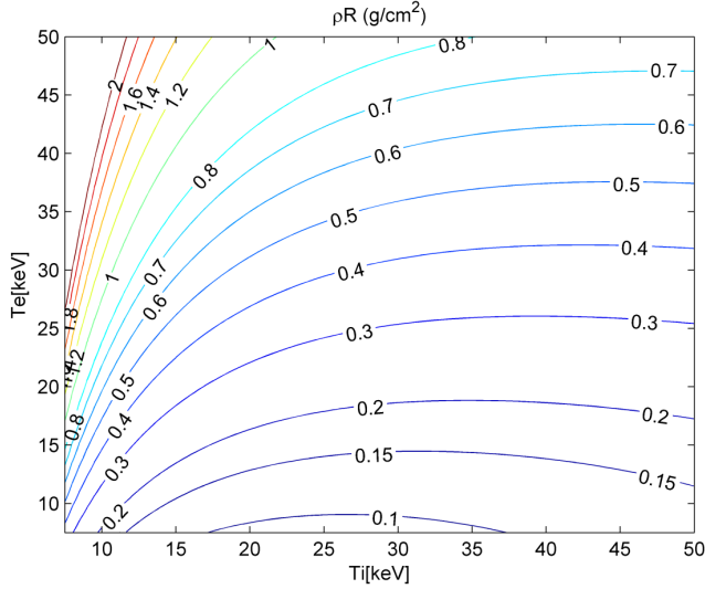
Figure 11. Contours of equal \rho \cdot R as a function of ions and electrons temperatures for DT.
