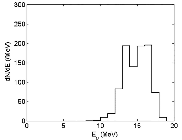
Figure 6. The measured secondary proton spectra in the shot with a target diameter of 800 \mu\text{m} .
