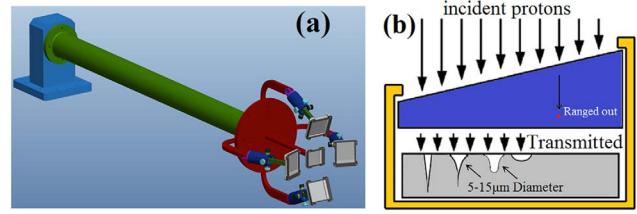
Figure 7. (a) The alignment of the Si-WRF spectrometer array at the SG-III facility (b) and a schematic illustration of a single WRF spectrometer [11] .
