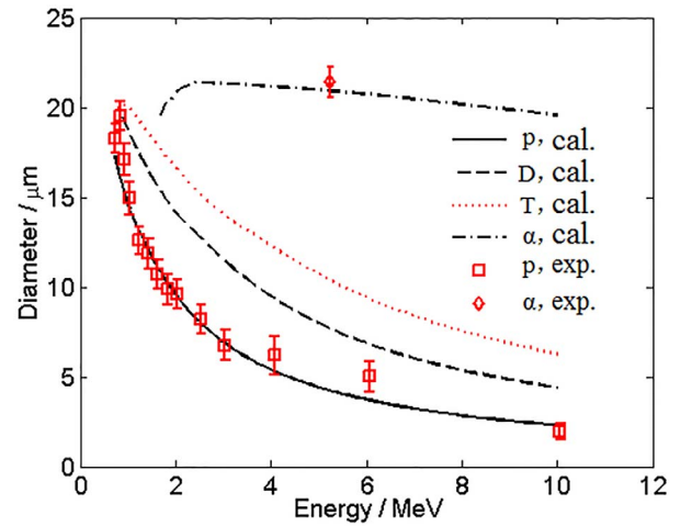
Figure 3. The measured and calculated energy responses of CR39 to proton, deuteron, triton and alpha.
