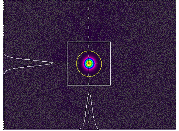
Figure 4. Far-field output beam profile of the 1018 nm SFS-YDFL.
