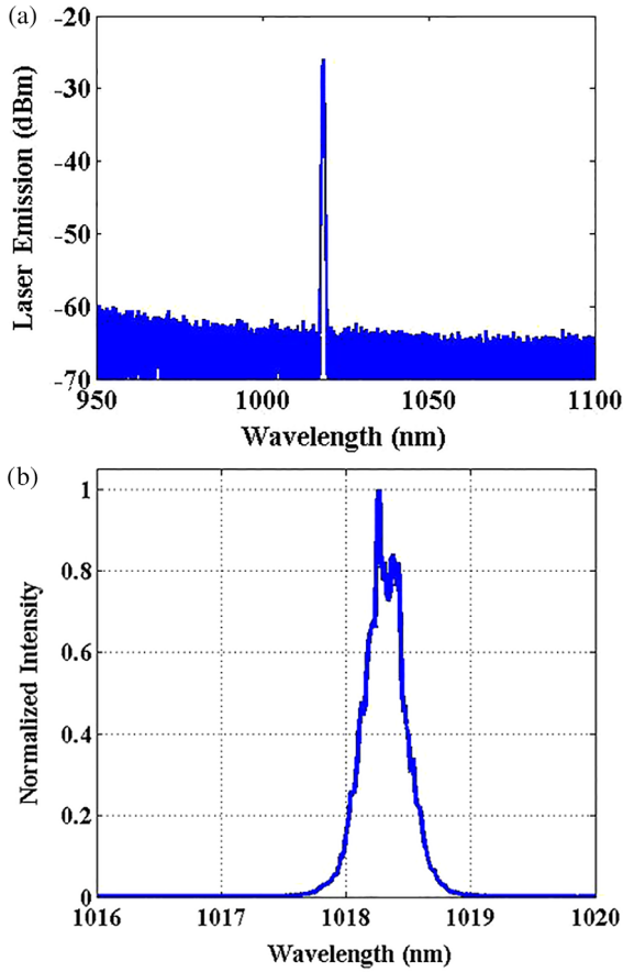
Figure 5. (a) Laser emission spectrum at different output powers, (b) laser emission spectrum at 100 W output power in linear coordinates.
