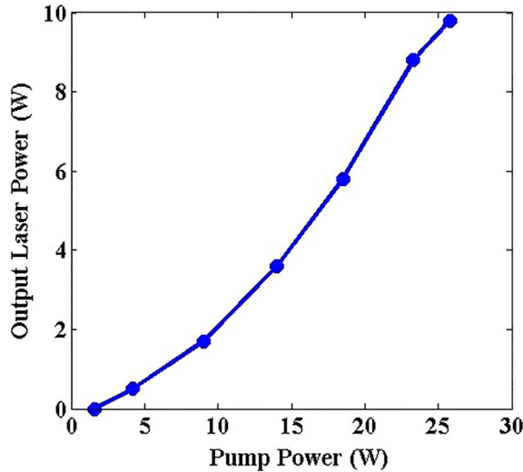
Figure 3. Laser output power versus pump power of the 10/125 \mu\text{m} fiber laser.
