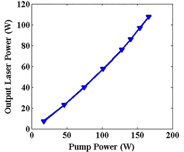
Figure 2. Laser output power versus pump power of the SFS-YDFL.
