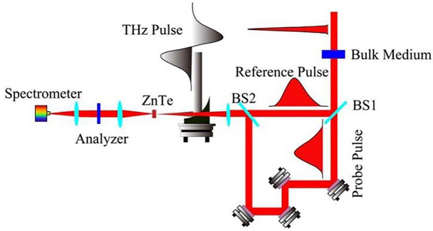
Figure 4. Spectral interferometry scheme using twin-chirped-pulse FDH (quoted from Ref. [28]).
