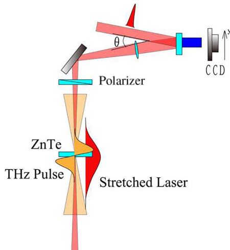
Figure 2. Schematic of ‘single-shot’ cross-correlation scheme.
