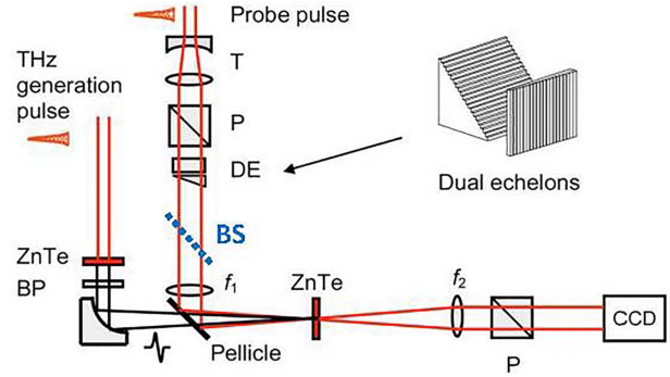
Figure 5. Schematic of single-shot THz measurement using dual echelon optics (quoted from Ref. [29]).
