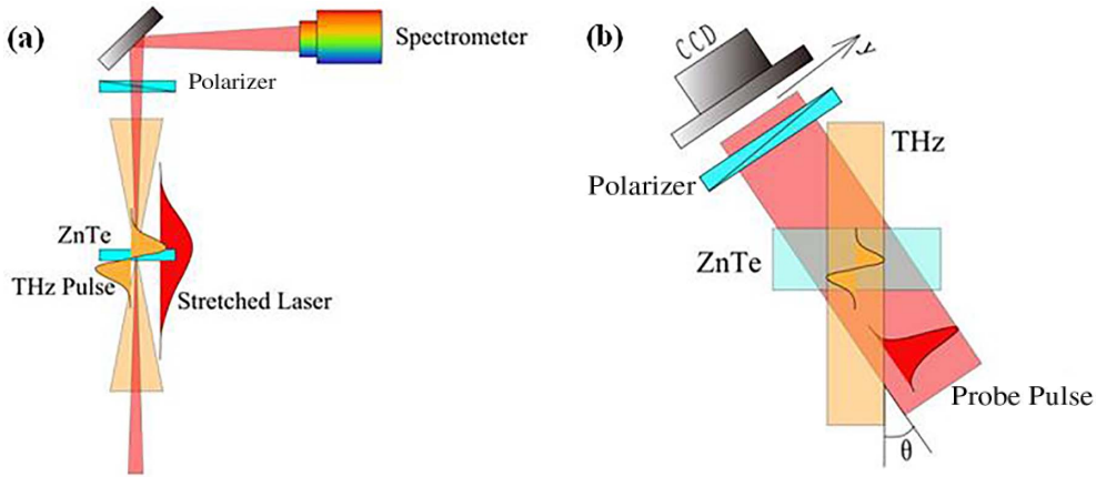
Figure 1. Schematic of (a) spectral encoding and (b) spatial encoding scheme.
