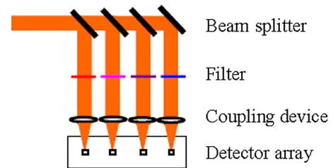
Figure 3. Schematic of a multi-channel THz-diagnostic system based on a direct detector array.
