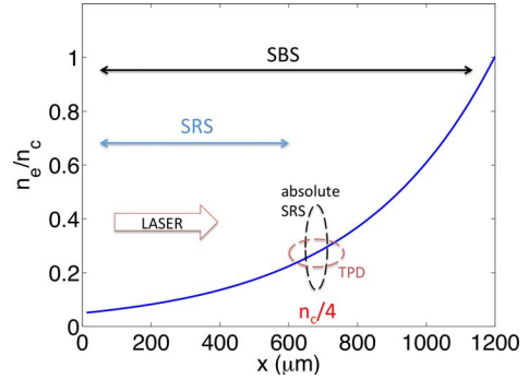
Figure 2. Localization of the various parametric instabilities in the plasma profile. The figure represents a realistic profile. The one used in the simulations is smaller (see Section 2).
