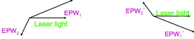
Figure 4. Geometry of the k -vectors involved in the TPD instability. The decay of a photon into two plasmons can be realized in two possible ways while preserving energy and momentum. This particular geometry applies in 2D and helps with the interpretation of the phase space diagrams. In reality, 3D, the number of possible k -vectors is infinite lying on an asymmetric cone around the laser k -vector.
