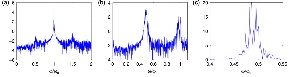
Figure 7. Frequency spectra for the cases (a) c8, (b) h9 and (c) a zoom of (b). Note: (a) and (b) are on log scale whereas (c) is on linear scale.
