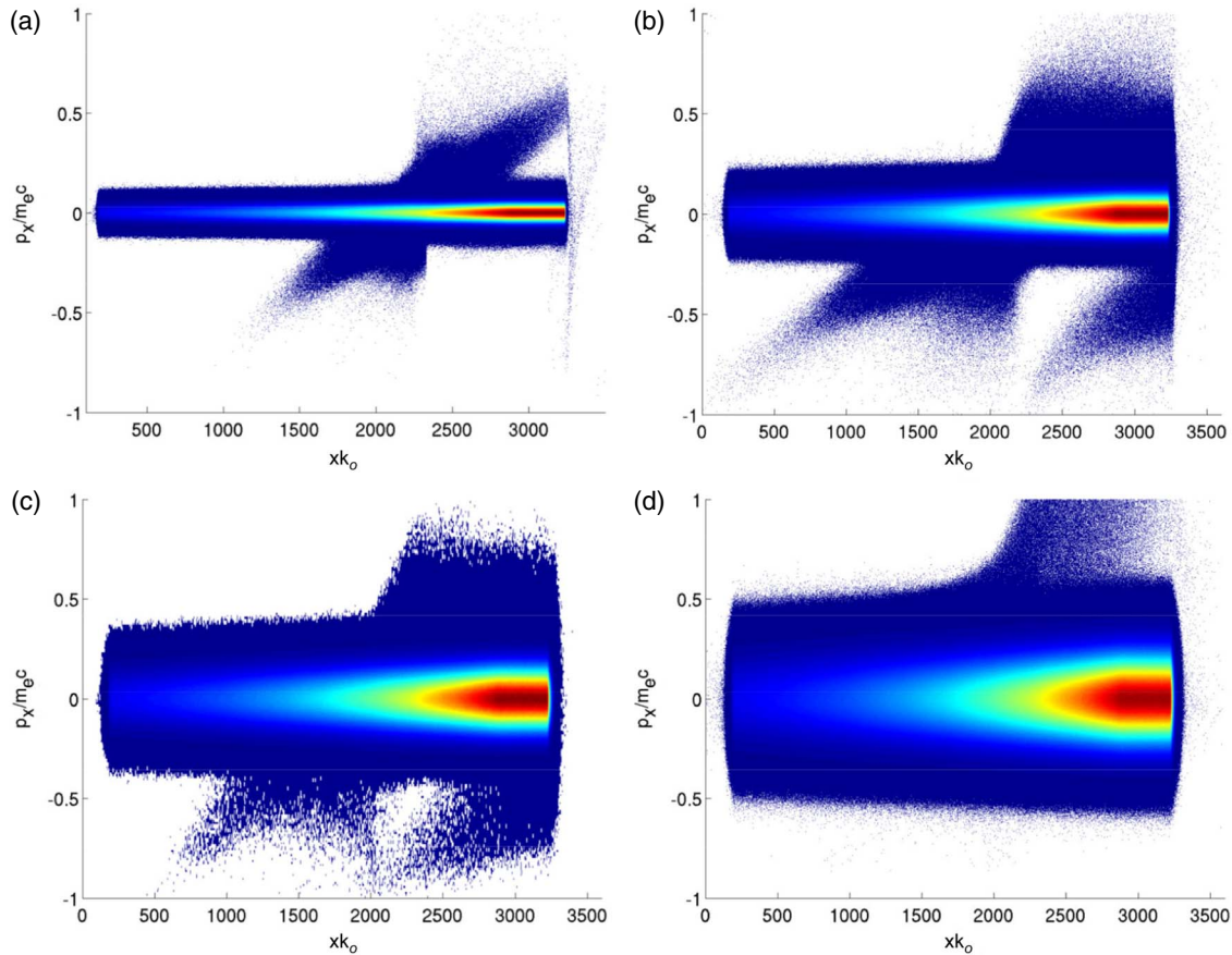
Figure 12. The transverse electron phase space as a function of the laser propagation direction for (a) case c8 at t\omega_o = 5600 , (b) case h8 at t\omega_o = 7000 , (c) case h7 at t\omega_o = 7400 and (d) case h9 at t\omega_o = 5200 . The time slice for h9 is taken at an early time as the electrons start to recirculate quickly.
