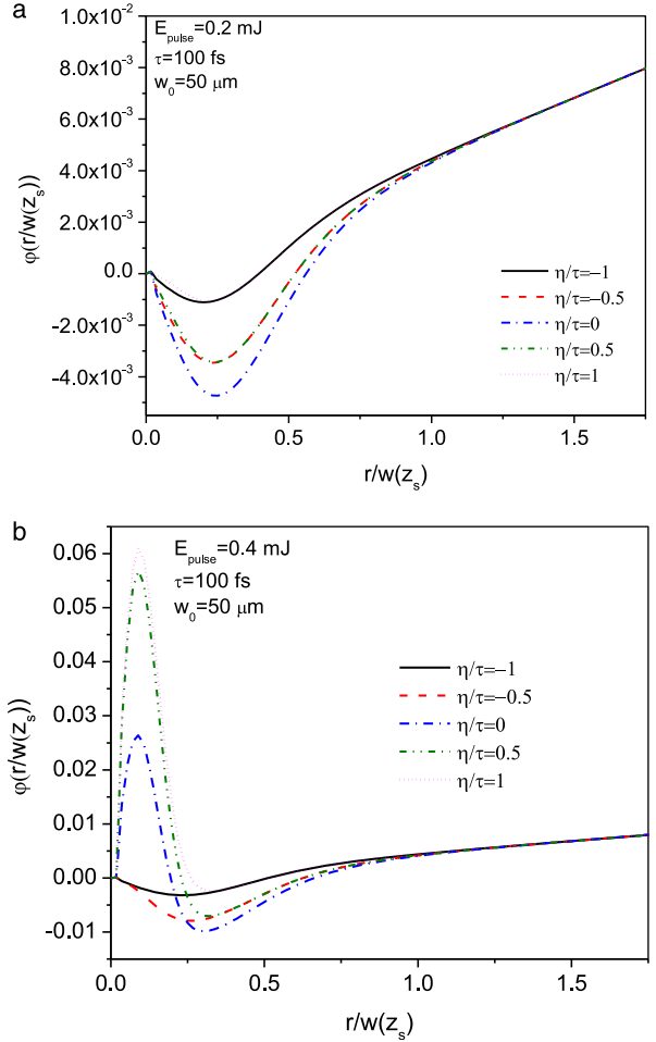
Figure 2. The angle of individual rays at the exit of the zone with high beam intensity where induced refraction is large computed for laser beam propagation through air (normal conditions) assuming Gaussian temporal shape of the laser pulse with duration \tau = 100 fs and a Gaussian spatial beam profile with the beam radius on 1/e^2 level in the waist, w_0 = 50 \mu\text{m} , shown as a function of dimensionless laser radius, r/w(z_s) , for different moments of dimensionless time, \eta/\tau , (negative – before the pulse): (a) total radiated energy per pulse E_{\text{pulse}} = 0.2 mJ (maximum irradiance I_0 = 2.87 \times 10^{17} \text{ W m}^{-2} ); (b) total radiated energy per pulse E_{\text{pulse}} = 0.4 mJ (maximum irradiance I_0 = 5.75 \times 10^{17} \text{ W m}^{-2} ). All computational results correspond to the laser wavelength \lambda = 800 nm.
