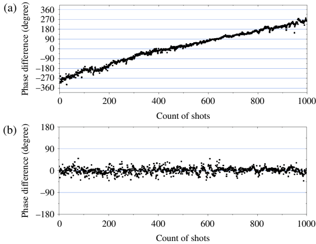
Figure 8. Experimental result of beam combination using an SBS-PCM and a feedback loop: (a) without operating the feedback loop and (b) with operation of the feedback loop.
