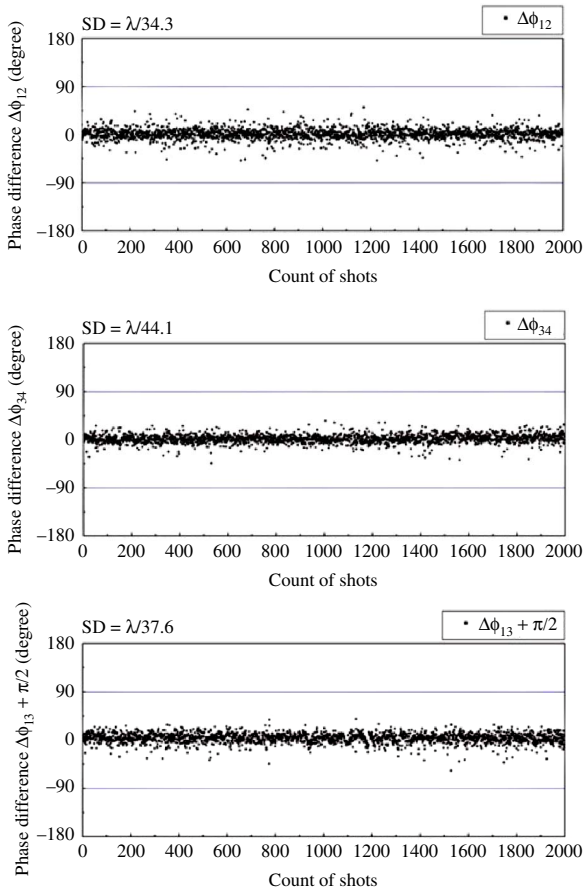
Figure 10. Measured phase fluctuation of four-beam combination using an SBS-PCM with the amplitude dividing method.
