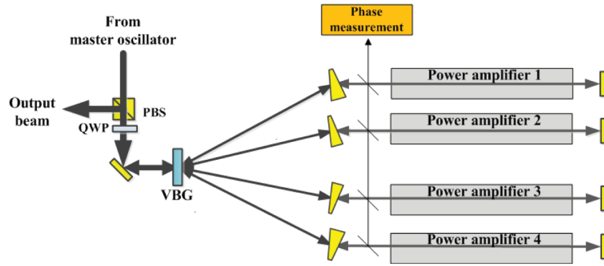
Figure 3. MOPA beam combination laser with the amplitude combining method using a VBG.
