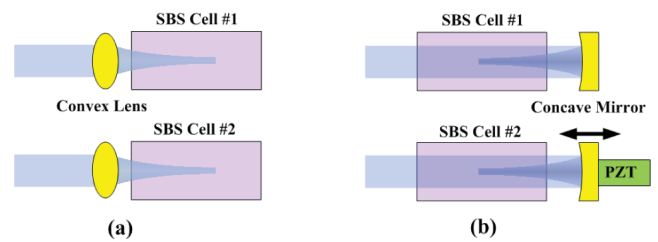
Figure 4. Types of SBS-PCM: (a) conventional SBS-PCM and (b) self-phase-locking SBS-PCM with PZT.
