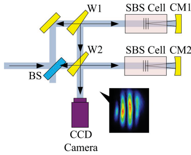
Figure 5. Experimental setup of the self-phase-locked SBS-PCM: BS, beam splitter; W1 and W2, wedges; CM1 and CM2, concave mirrors.
