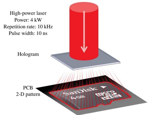
Figure 16. Schematic diagram of 2D laser processing using the Kumgang laser.
