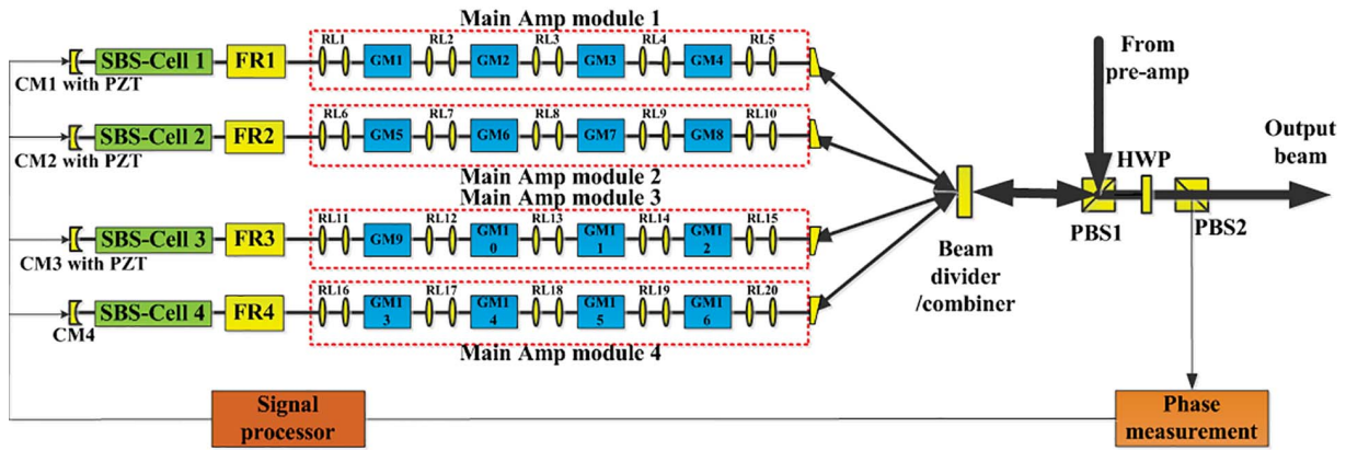
Figure 15. Schematic diagram of the main amplifier: RL1–RL20, relay lens pairs; CM1–CM4, concave mirrors.
