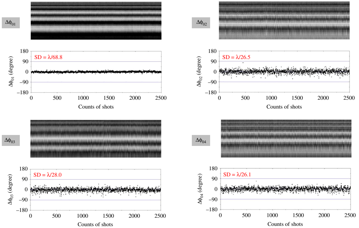
Figure 12. Measured phase fluctuation of the four-beam combination amplifier using an SBS-PCM with the wavefront dividing method.
