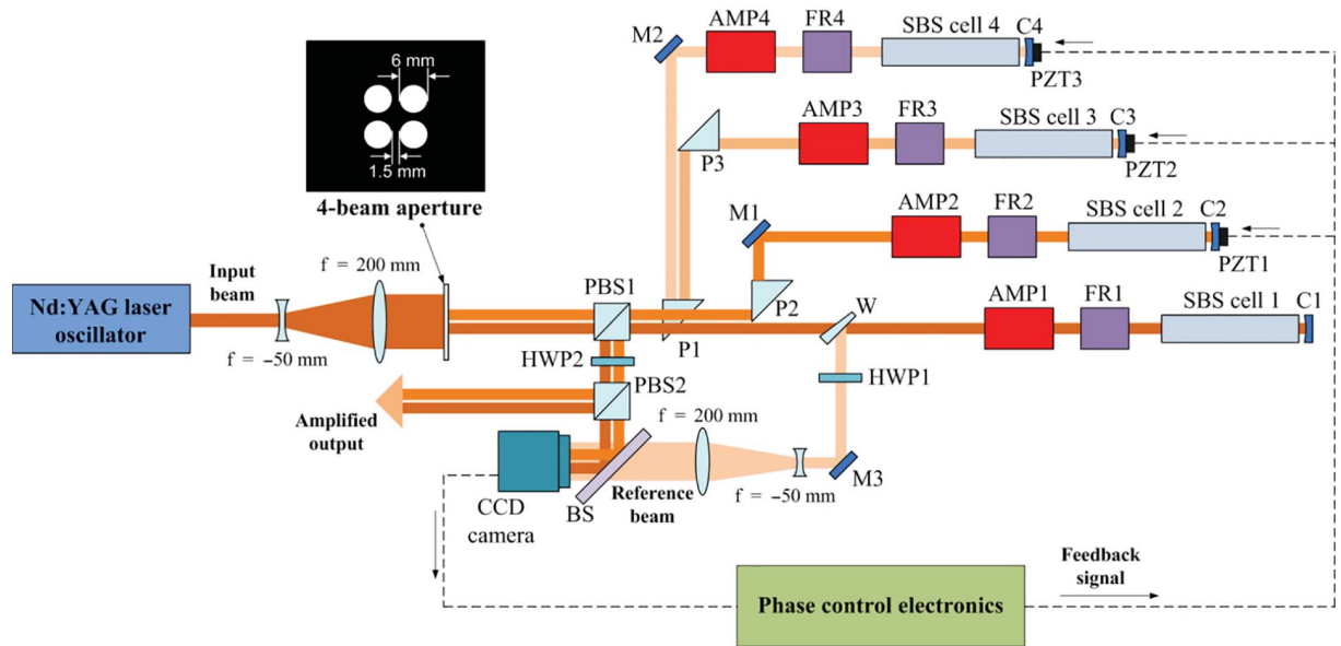
Figure 11. Experimental setup of the four-beam combination amplifier using an SBS-PCM with the wavefront dividing method: HWP1 and HWP2, half-wave plates; BS, beam splitter; P1–P3, Prisms; M1–M3, mirrors; AMP1–AMP4, amplifiers; C1–C4, concave mirrors; W, wedge.
