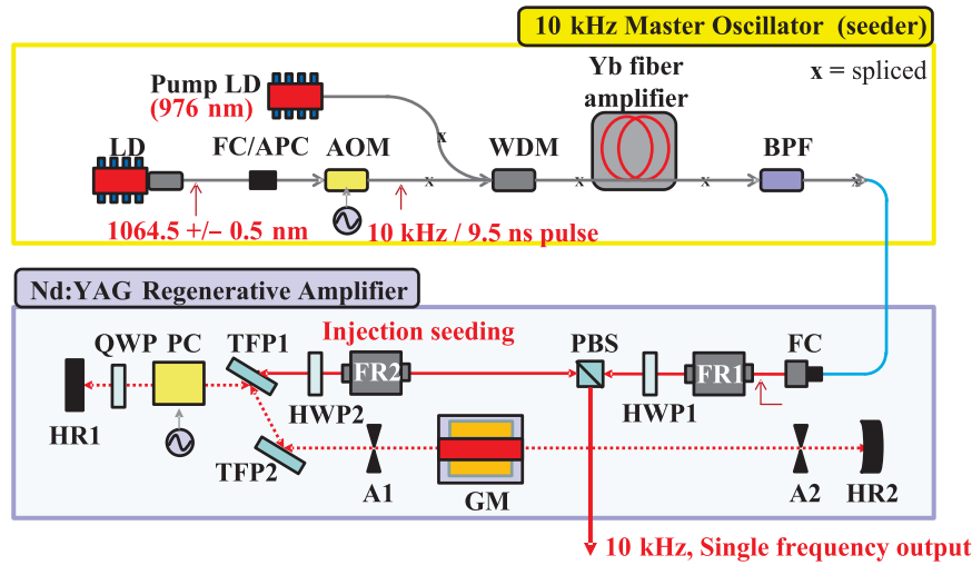
Figure 13. Schematic diagram of the front end: FC/APC, fiber connector/angled physical contact; WDM, wavelength division multiplexor; BPF, bandpass filter; FC, fiber collimator; HR1 and HR2, high-reflectivity mirrors; A1 and A2, apertures.
