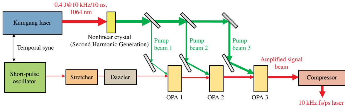
Figure 17. Schematic diagram of the generation of a fs/ps laser using the Kungang laser as a pump source: OPA1–OPA3, optical parametric amplifiers.
