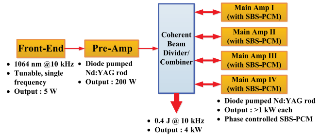
Figure 1. The schematic diagram of the Kumgang laser system.
