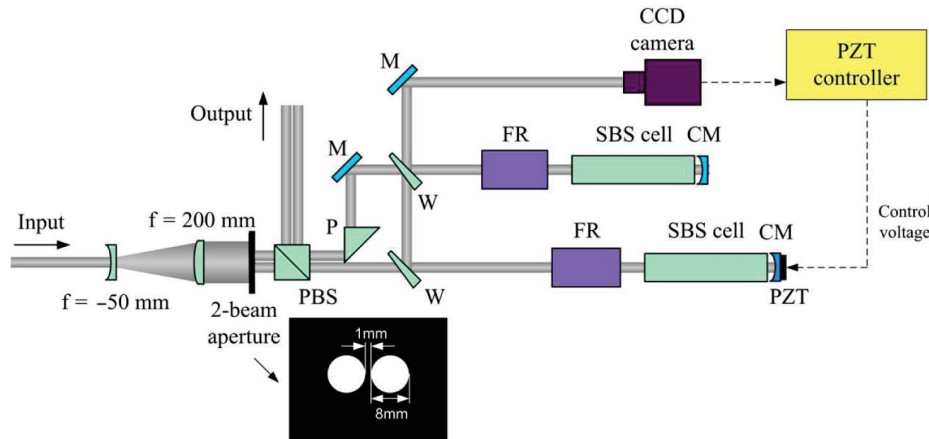
Figure 7. Experimental setup of beam combination using an SBS-PCM and a feedback loop: M, mirror; W, wedged window; CM, concave mirror.
