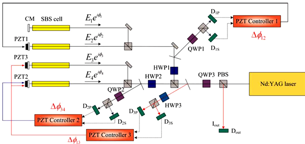
Figure 9. Experimental setup of the four-beam combination using an SBS-PCM with the amplitude dividing method: D_{1P} , D_{1S} , D_{2P} , D_{2S} , D_{3P} , D_{3S} and D_{out} , energy detectors; CM, concave mirror.
