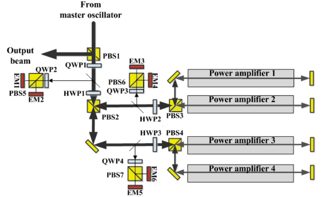
Figure 2. The MOPA beam combination laser with the amplitude combining method using PBS: EM1–EM6, energy meters.
