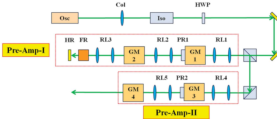
Figure 14. Schematic diagram of the pre-amplifier: RL1–RL5, relay lens pairs; PR1 and PR2, polarization rotators; HR, high-reflectivity mirror.
